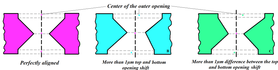
Figure 9. Simplified side view of the B and C GEM foil hole categories. See figure 3 for an A category GEM foil hole.
