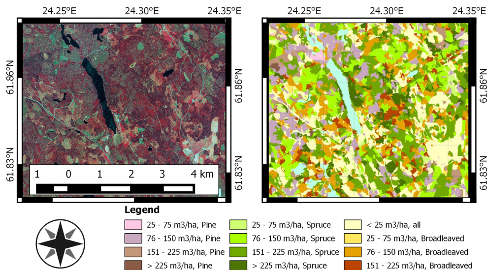
Figure 9. GeoEye color-infrared image (Near-Infrared Red Green) acquired on 7 July 2010 in Hyytiälä, Finland ( left ), and the growing stock volume map ( right ) trained with Relasphone biomass data as the reference. Reproduced with permission from IIEE.
