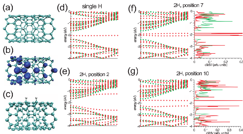
Figure 4. Electron densities and band structures for a (10,0) nanotube with one and two H adatoms. (a) Atomic structure with a single H adatom, top view. Electron density near the Fermi level (energy interval 0.7 eV) is shown in (b) for the same tube. (c) (10,0) nanotube with two nearby adatoms, side view. (d) Band structure of a nanotube with single adatom and (e) two adatoms in positions (see figure 5) 0 and 2. (f) Band structure and LDOS near two H adatoms in positions 0 and 7. (g) The same for two H adatoms in positions 0 and 10.
