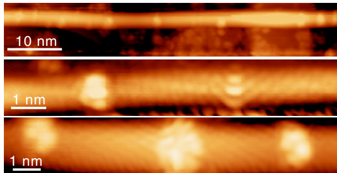
Figure 1. STM topography images of SWNTs deposited on a Au(111) surface, with hydrogen plasma-induced defects forming hillock-like protrusions with apparent heights comprised between 1 and 3 Å. Typical measurement parameters are U_s = 1 V, I_s = 0.1 nA.
