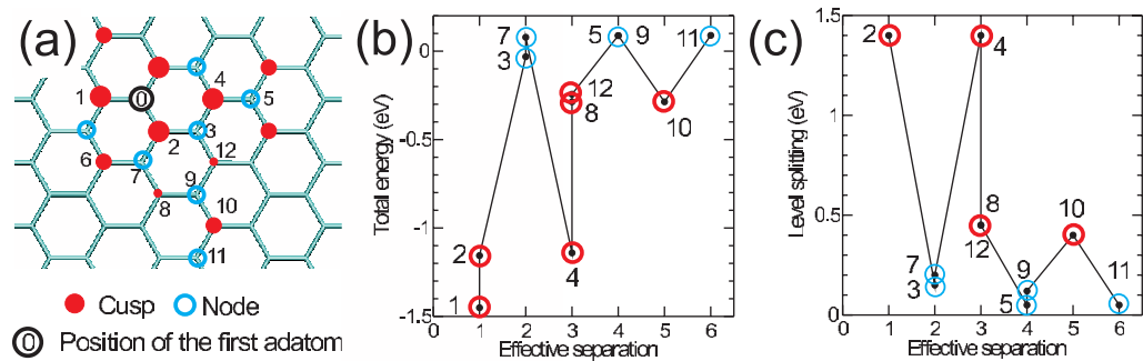
Figure 5. First-principles simulations for a (10,0) SWNT with H adatoms. (a) The adsorption sites of H adatoms. All positions are metastable (separated by energy barriers from each other) so that all of them can exist at low experimental temperatures. The red and blue circles reflect the nodal structure of electron density oscillation near the Fermi energy when there is a single adatom on site labeled ‘0’. (b) The total energy of the system for different positions of the second adatom. The separation between adatoms is defined as the number of bonds in graphene lattice on the migration path of the second adatom to arrive at site ‘0’. (c) The splitting of the H-induced levels in the gap due to adatom–adatom interaction.
