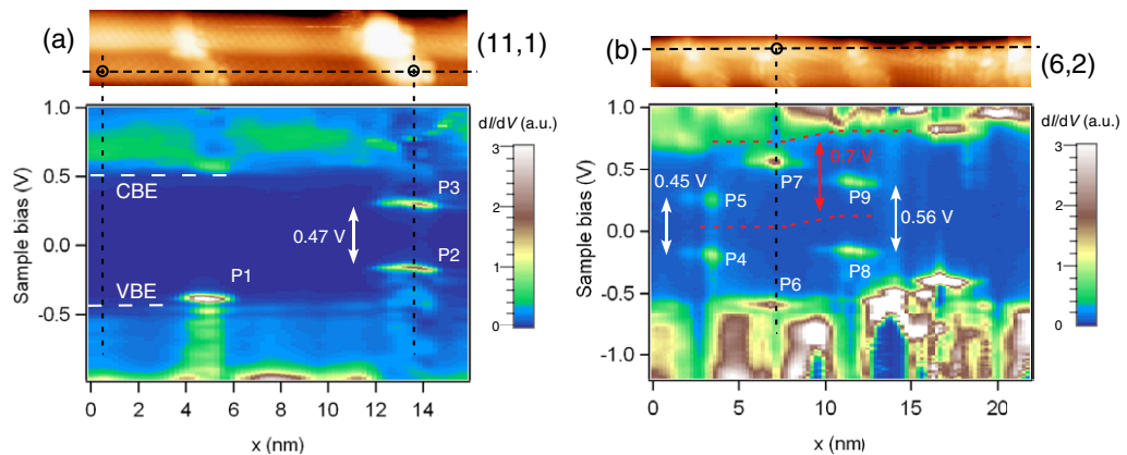
Figure 2. STM topography images of SWNTs treated with low-energy hydrogen plasma on a gold (111) substrate and the corresponding dI/dV color-scale contour maps (lower panels) for two nanotubes. The spectra were recorded along the dashed horizontal lines. A sharp single peak (P1) at the VBE and a pair of peaks (P2–P3) positioned symmetrically relative to the bandgap edges are visible in (a). FWHM of P1, P2 and P3 are 28, 26 and 33 meV, respectively. (b) Shows three defect-induced symmetric double peak structures with different energy separations. FWHM of P4, P5, P6, P7, P8 and P9 are 93, 125, 79, 84, 67 and 73 meV, respectively. Measurement parameters in (a): U_s = 1 V, I_s = 0.6 nA, T = 5.56 K, U_{\text{mod}} = 6 mV, x_{\text{res}} = 0.21 nm; (b): U_s = 1 V, I_s = 0.3 nA, T = 5.36 K, U_{\text{mod}} = 10 mV and x_{\text{res}} = 0.22 nm.
