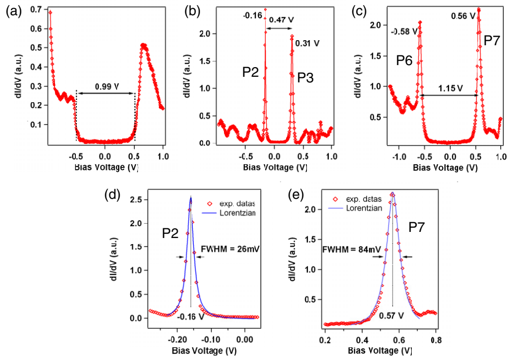
Figure 3. Comparison of spectroscopic signatures of individual point defects. dI/dV plots correspond to the positions indicated by small circles for the (11,1) SWNT shown in figure 2(a), related to the pristine nanotube (a) and the defected structure (b), respectively. (c) The same for the (6,2) SWNT, figure 2(b). P2 and P7 peaks fitted with a Lorentzian function, (d) and (e), respectively.
