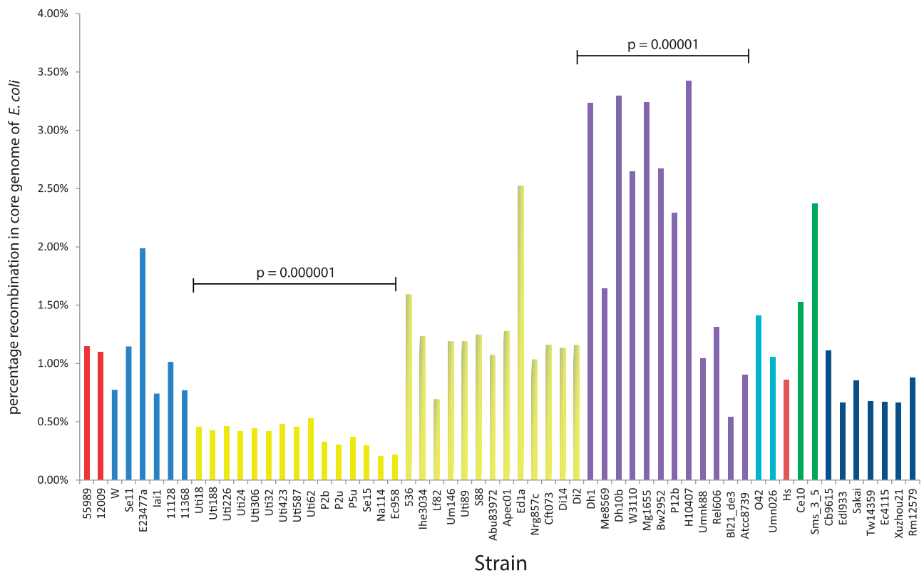
Fig. 5. —Graph showing the percentage of core genome undergoing recombination in each of the 62 genomes in our analysis. Bars are color coded according to the BAPS cluster that strain is allocated to (yellow = BAPS 4; light yellow ST131 strains within BAPS 4; brown = BAPS 7; purple = BAPS 5; light blue = BAPS 3; red = BAPS 1; dark blue = BAPS 9; cyan = BAPS 6; green = BAPS 8). Bars with values above the ST131 and K12 strains indicate P values for significant difference between that group of strains and all others as determined by standard permutation tests.
