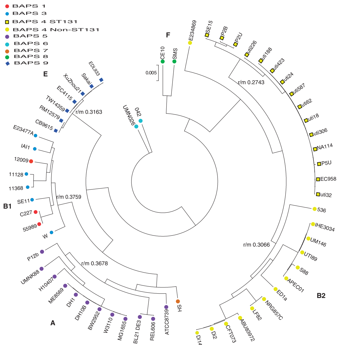
FIG. 1. —Whole-genome-based phylogeny of Escherichia coli . The phylogeny is based on approximately 2.3-Mbp core genome aligned using Mugsy, with an ML phylogeny determined using RAxML. Classical phylogroup is indicated at each clade of the tree with the appropriate capital letter. Strains are further color coded according to allocated BAPS cluster (yellow = BAPS 4, ST131 isolates with black border; brown = BAPS 7; purple = BAPS 5; light blue = BAPS 3; red = BAPS 1; dark blue = BAPS 9; cyan = BAPS 6; green = BAPS 8). The calculated r/m value for each major clade is also presented.
