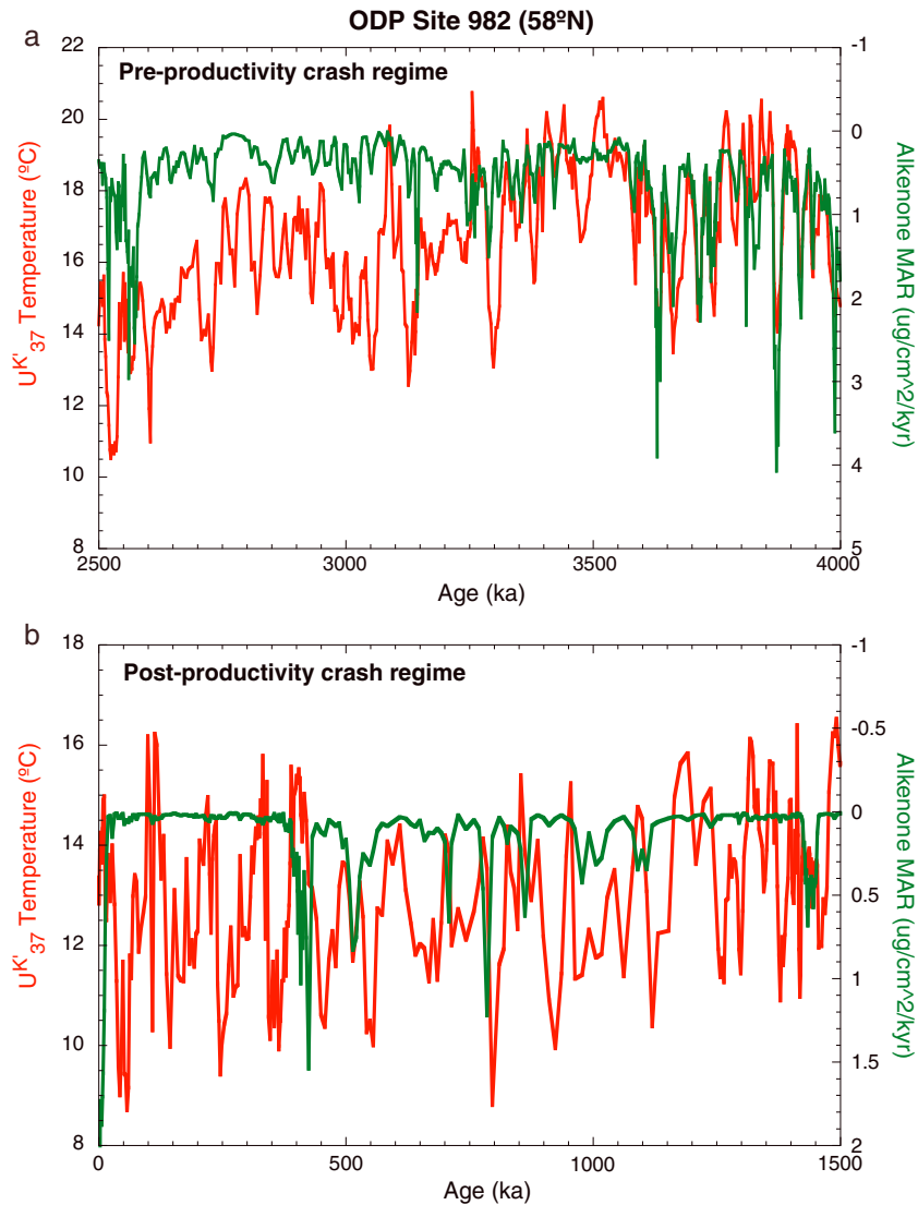
Figure 4. ODP site 982 Surface Conditions. North Atlantic sea surface temperature (red) [Lawrence et al. , 2009] and C 37 alkenone MAR (µg/cm 2 /kyr) data (green) [Bolton et al. , 2011] from ODP site 982 (58°N, 16°W) for: (a) preproductivity crash regime (4 to 2.5 Ma) and (b) postproductivity crash regime (1.5 to 0 Ma). Note the axis is inverted for the C 37 alkenone MAR data.
