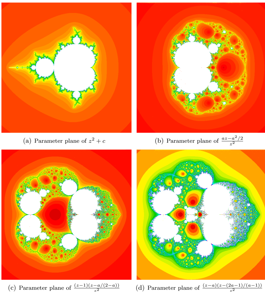
Figure 3: The slices \text{Per}_1(0), \text{Per}_2(0), \text{Per}_3(0) and \text{Per}_4(0)
