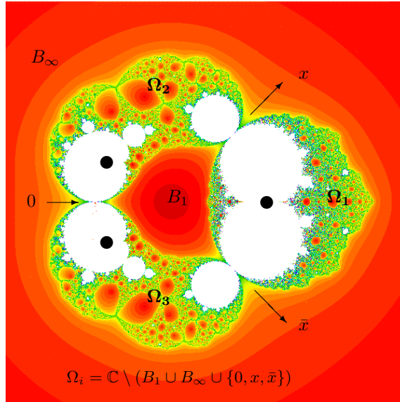
Figure 8: The slice Per_3(0) .
