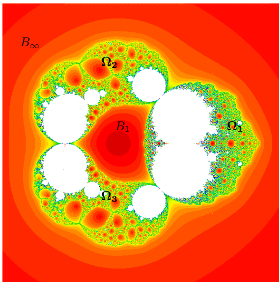
Figure 4: The slice Per_3(0) and its pieces.
