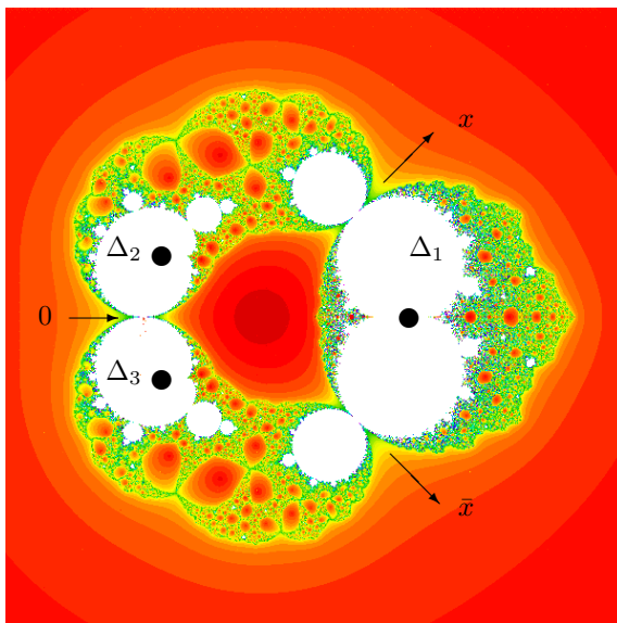
Figure 10: The slice Per_3(0) .
