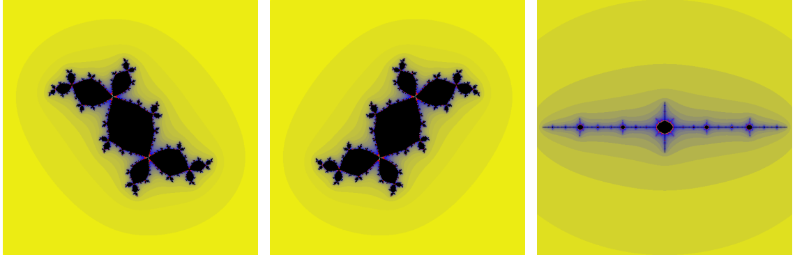
(a) The Douady rabbit. The Julia set of z^2 - 0.122561 + 0.744861i . (b) The Douady co-rabbit. The Julia set of z^2 - 0.122561 - 0.744861i . (c) The airplane. The Julia set of z^2 - 1.75488 .
