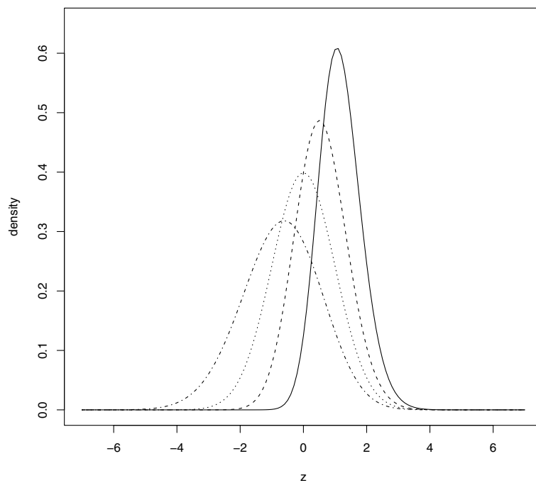
Figure 1: Density \varphi_Z(z; \alpha) for \alpha equals to 5 (solid line), 2 (dashed line), 1 (dotted line) and 0.5 (dash-dot line).
