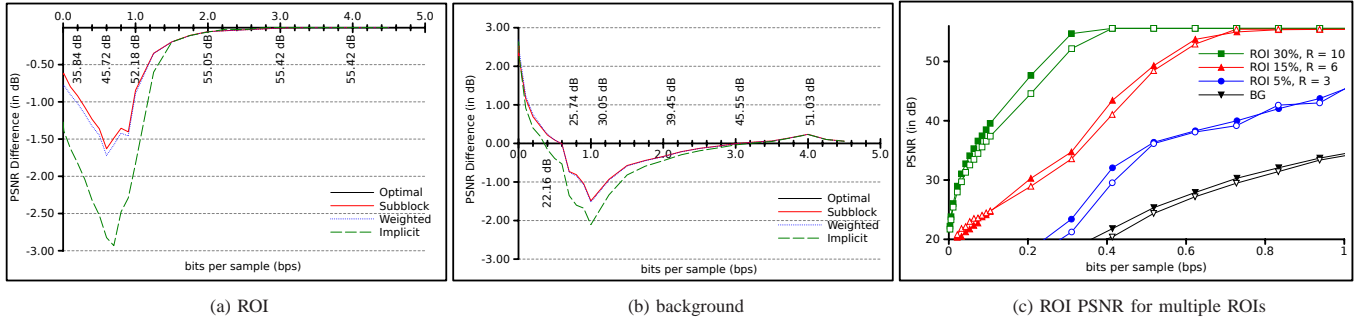
Figure 2. Average coding performance of the ROI area for the eight images of the ISO 12640-1 corpus. Evaluation of the coding performance achieved by Subblock, Weighted, Implicit, and theoretical Optimal. Results are for ROI priority average, for \mathcal{R} from 3 to 8 for all methods. (a) PSNR differences of the ROI area, for single ROI. (b) PSNR differences of the background, for single ROI. (c) PSNR of the ROI area, for multiple ROIs.
