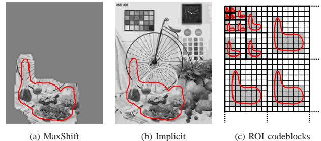
Figure 1. Bicycle image (size 2048 \times 2560 , gray-scaled) decoded at a target bitrate of 0.01 bps, with a ROI (emphasized in the graphic in red) prioritized at \mathcal{R} = 15 .
