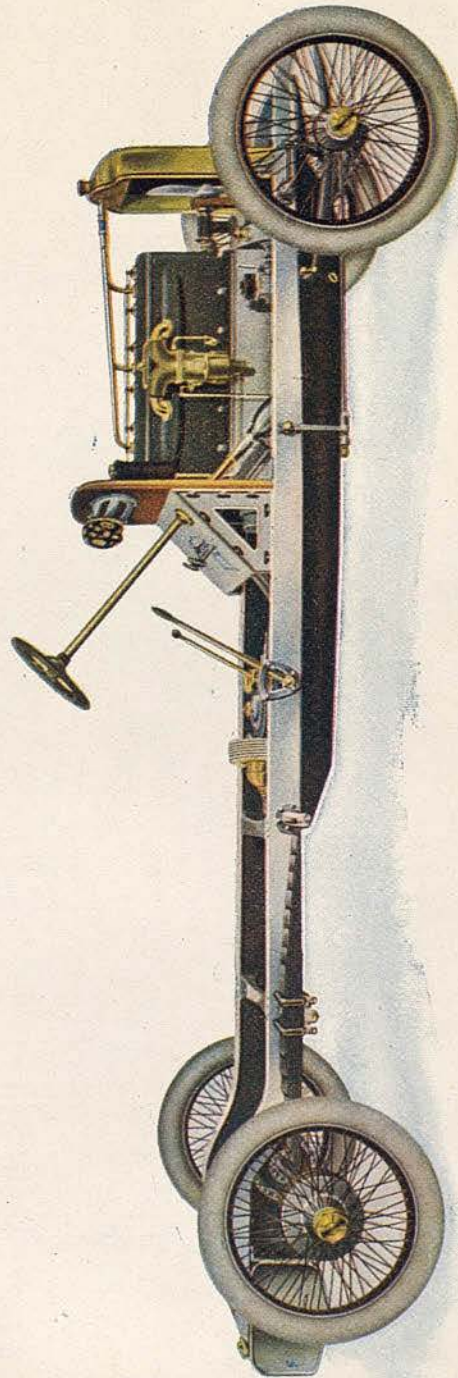
Chassis Minerva 30 HP (6 cilindres)
