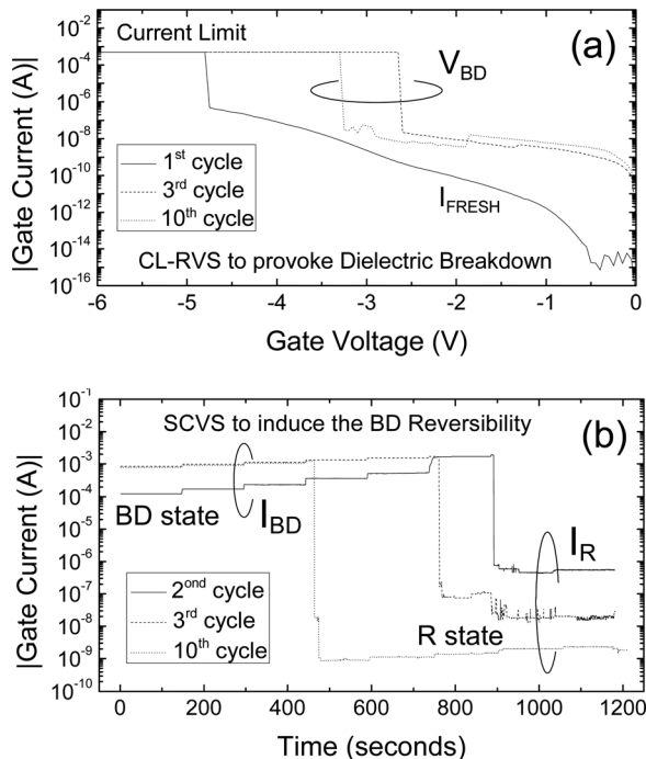
Fig. 2. Gate current recorded (a) during the CL-RVS necessary to reach the BD state and (b) during the SCVS necessary to provoke the BD recovery (R-state).
