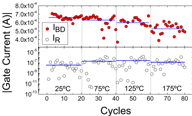
FIG. 4. (Color online) I_G evolution with cycling after BD transient (colored circles) and after BD recovery (open circles). Every 20 cycles the temperature was increased by 50°C, starting from 25°C until 175°C is reached. Blue lines indicate the mean values at each temperature.
