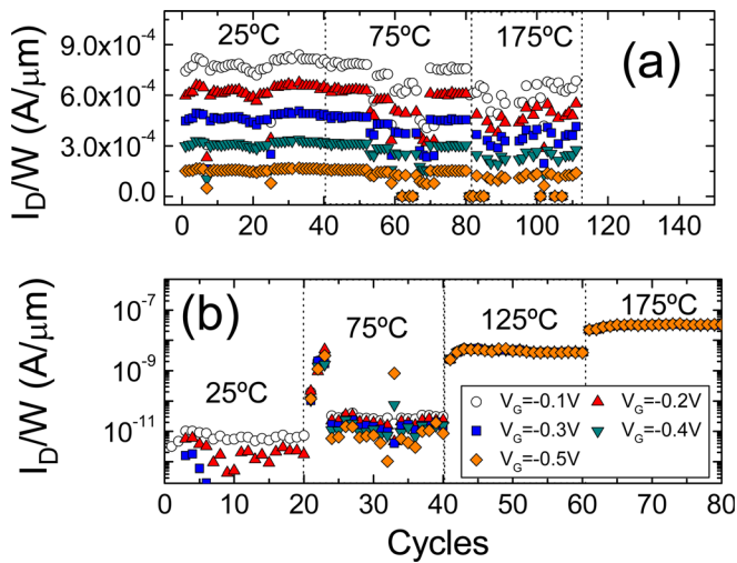
FIG. 6. (Color online) Drain current measured at different temperatures in devices after BD, when the conductive path is located close to drain (a) or source (b).
