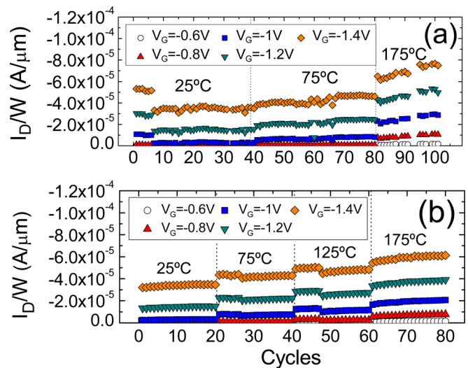
FIG. 7. (Color online) Drain current (normalized to the transistor width) measured at different temperatures in devices after the BD recovery when the conductive path is located at the drain (a) or source (b). Similar currents are measured in both cases which state that after recovery the BD path location has no relevant influence in the transistor electrical characteristics.
