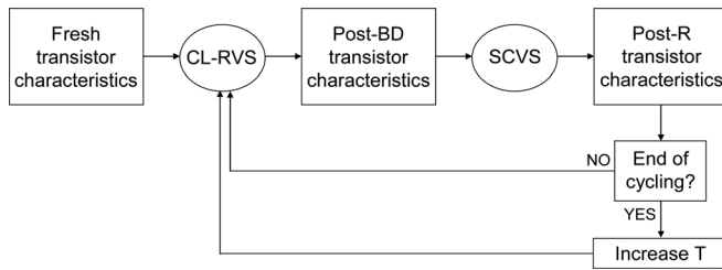
Fig. 1. Stress-measurement sequence designed to analyze the dielectric BD reversibility. The compliance of the measurement equipment was used to limit the current during current-limited stress (CL-RVS).
