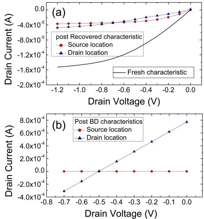
FIG. 5. (Color online) Drain current versus drain voltage measured for (a) fresh and recovered devices, with BD paths located close to drain or source and (b) after inducing the BD in the same samples.
