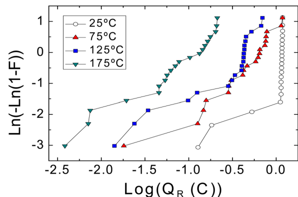
Fig. 3. (Color online) Statistical distributions of the Q_{\text{R}} measured during cycling on the same sample. The “F” function represents the cumulative probability function of Q_{\text{R}} . Distributions are organized by temperature, which was increased by 50^\circ\text{C} every 20 cycles in the same sample.
