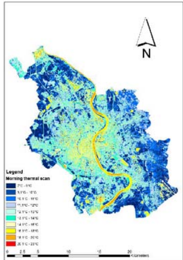
Figure 2.3. Morning thermal scan of Cologne (July 1 st 1995 at 4 a.m.) (Source: Environmental Department of Cologne)
