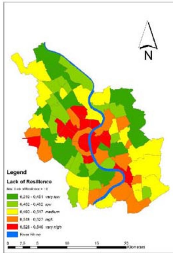
Figure 2.18. Spatial distribution of the lack of resilience of the population of Cologne to heat waves per city district.
