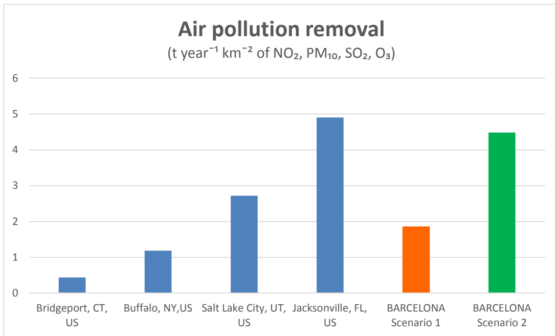
Figure 3.6. Air pollution removal potential, in \text{t year}^{-1} \text{ km}^{-2} of \text{NO}_2 , \text{PM}_{10} , \text{SO}_2 , \text{O}_3 derived for different cities from the literature (see Table 3.3) and from the results obtained for Barcelona scenarios 1 and 2 (Table 3.2).
