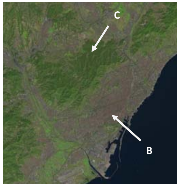
Figure 3.1. Landsat image of Barcelona city (B) and Collserola (C) areas. (Source: LandsatLook, USGS)
