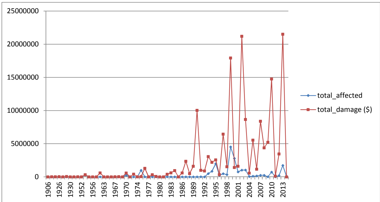
Figure 0.1. Total number of persons affected and total damages (US$) due to climatological, meteorological and hydrological hazards in Europe between 1900 and 2014 (Data source: International Emergency Disasters Database, EM-DAT, http://www.emdat.be/ ).
