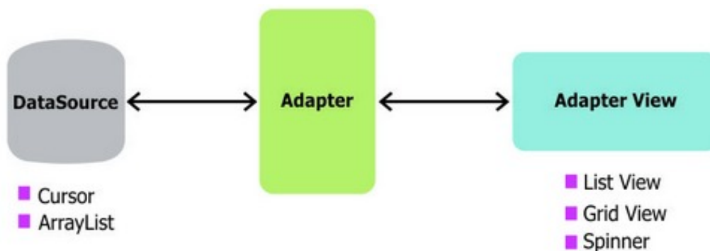
Figura 2.3: Diagrama Adapter
