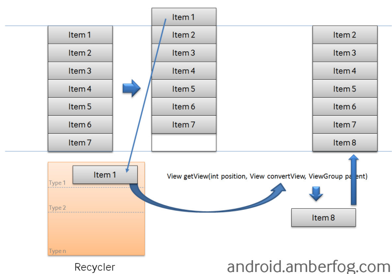
Figura 2.4: Android Recycler
