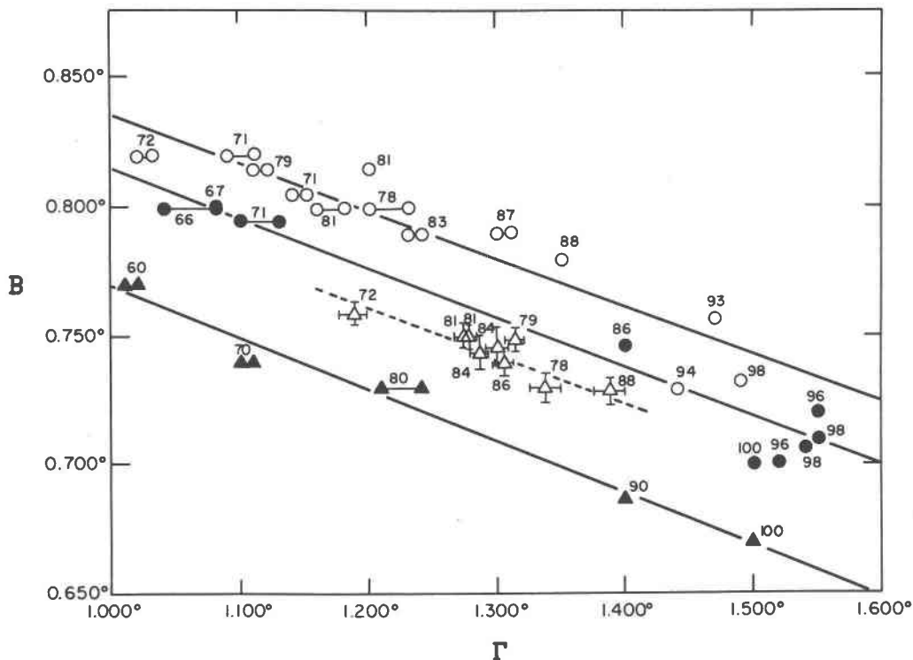
FIG. 1. A plot of B(2\theta_{(1\bar{1}1)} - 2\theta_{(\bar{2}01)}) versus \Gamma(2\theta_{(131)} + 2\theta_{(220)} - 4\theta_{(131)}) for calcic plagioclases. The feldspars have been grouped into 4 groups on the basis of their origin, with the following symbols: \circ (hypabyssal, plutonic, pegmatitic, metamorphic, charnockitic, and those from large basic igneous complexes); \bullet (volcanic); \triangle (volcanic ash layers); and \blacktriangle (synthetic). All data, except for the data on volcanic ash layers, was taken from Smith and Gay (1957). Diagonal lines represent regression lines through the various groups of data. Vertical and horizontal lines drawn through symbols for volcanic ash plagioclases represent plus and minus two standard deviations on the means of B and \Gamma , respectively. Horizontal lines connecting two symbols represent those samples for which more than one \Gamma value was given by Smith and Gay. Numbers above symbols denote wt percent An_{(An+Ab)} .
