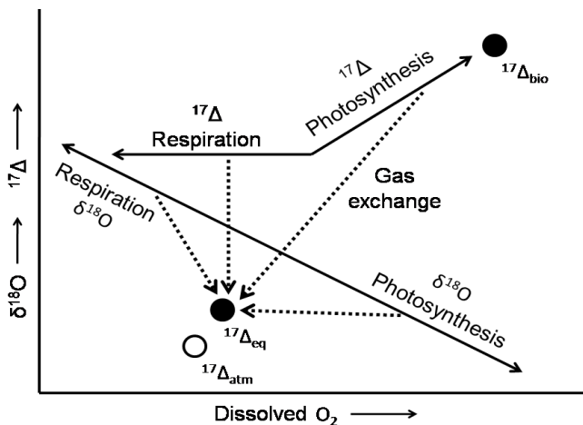
Figure 5. A schematic diagram showing the effects of photosynthesis, respiration, and air–water gas exchange on dissolved O_2 concentrations, \delta^{18}O and ^{17}\Delta . \delta^{18}O changes with all the processes and additionally is also affected by mixing. Because of non-mass-dependent processes occurring in the stratosphere, the ^{17}\Delta of O_2 in air has a different signal to the O_2 produced biologically where fractionation is mass-dependent. ^{17}\Delta increases due to photosynthesis, decreases due to gas exchange but is not affected by respiration. Respiration removes O_2 and decreases the dissolved O_2 concentration but fractionates O_2 isotopes in a mass-dependent way, which does not affect the relative proportion of \delta^{17}O and \delta^{18}O and therefore the ^{17}\Delta . ^{17}\Delta_{bio} is the maximum value of pure biological signal, which amounts to ^{17}\Delta of water. The slope of ^{17}\Delta increase towards ^{17}\Delta_{bio} is the kinetic slope \lambda for respiration ( \lambda = 0.518 ). ^{17}\Delta_{eq} is the O_2 at air–water equilibrium, which has a small offset from ^{17}\Delta_{atm} , which is by definition 0, due to fractionation at equilibrium where \delta^{17}O and \delta^{18}O slopes during invasion and evasion follow a slightly different slope to that of respiration.
