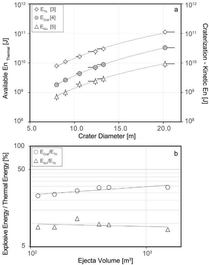
Fig. 9. (a) Semi-log plot showing thermal ( E_{Th} ), craterisation ( E_{Crat} ) and kinetic ( E_{Kin} ) energy vs. crater size (see also Table 1). (b) Log-log plot showing the ratio of craterisation and kinetic energy to thermal energy.
