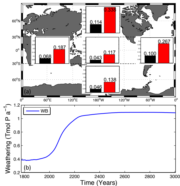
Figure 3: (a) Phosphorus weathering input (in \text{Tmol a}^{-1} ) into the Pacific Ocean (middle), Atlantic Ocean (right, middle), Indian Ocean (left, middle), Northern Oceans (=oceans north of 30^\circ \text{ N} ; upper middle) and Southern Ocean (=ocean south of 30^\circ \text{ S} ; lower middle) in 1775 (black bars) and 3005 (red bars). 30^\circ \text{ N} and 30^\circ \text{ S} constitute the separating line of calculations. (b): Annual mean averaged phosphorus weathering input (global sum) of 1775 until year 3005.
