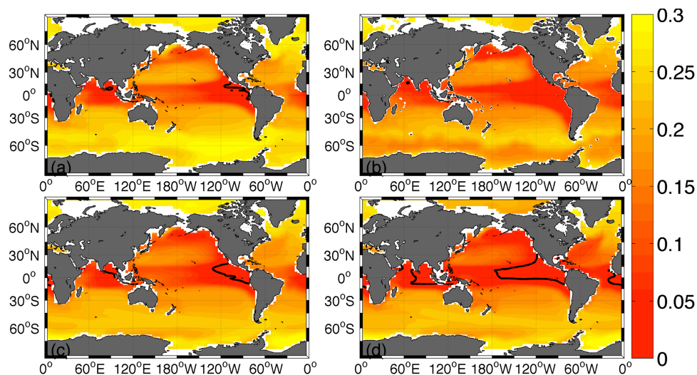
Figure 5: Oxygen concentration in \text{mol O}_2 \text{ m}^{-3} at 300m depth simulated by the (a) control simulation at year 1775 (representative for both REF and WB model runs in year 1775), (b) the World Ocean Atlas in 2009, (c) the control simulation at year 3005 and (d) simulation WB at year 3005. The black isoclines at 0.005 \text{ mol m}^{-3} highlight the oxygen minimum zones (OMZs).
