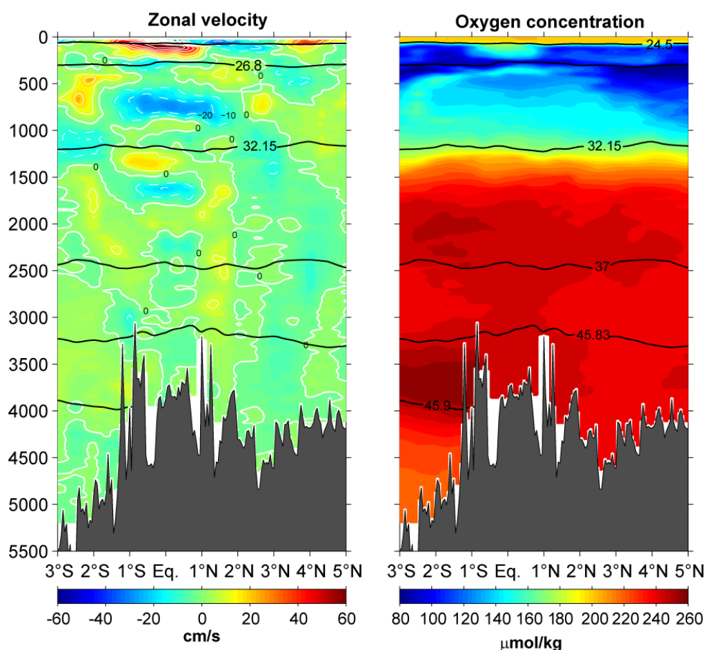
Abb. 1: Zonal velocity in cm/s (left panel) and concentration of dissolved oxygen in \mu\text{mol/kg} (right panel) between 3°S and 5°N along 23°W. (Plot: Marcus Dengler)
