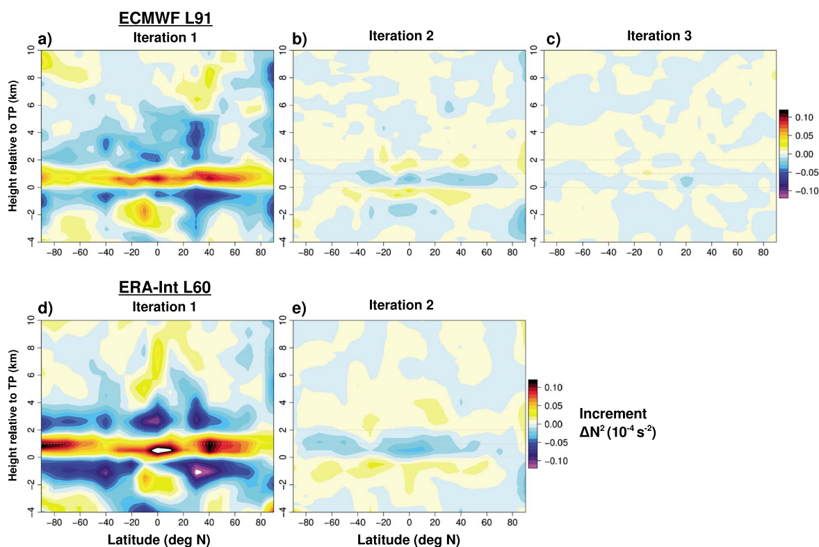
Figure 2. Zonal-mean, tropopause-based N^2 increments over successive iterations of the 4D-Var assimilation procedure for (a–c) the ECMWF L91 forecast model and (d, e) the ERA-Interim reanalysis. Averaged for January 2010. For orientation, grey dashed lines denote the tropopause and +1/+2 km.
