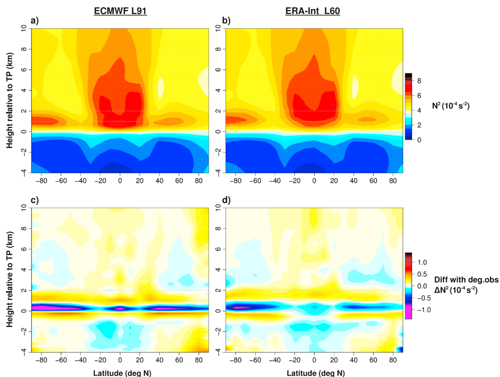
Figure 1. Latitude-height sections of tropopause-based zonal-mean N^2 in (a) the ECMWF L91 forecast model and (b) the ERA-Interim reanalysis. The bottom row differences from observations degraded to (c) the pressure of ECMWF’s 91 model levels and (d) the pressure of ERA-Interim’s 60 model levels. Averaged for January 2010. For orientation, grey dashed lines denote the tropopause and +1/+2 km.
