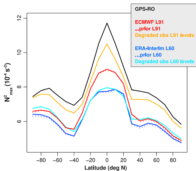
Figure 3. Zonal-mean TIL strength over all latitude bands measured as N^2_{\max} . The color lines corresponding to the different data sets are shown in the top right corner. Averaged for January 2010.
