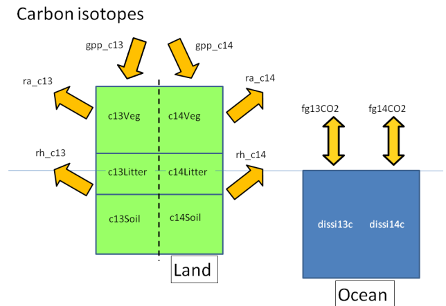
Figure 17. Carbon isotope diagnostics. Only report for models simulating isotopes. We define c13Land = c13Veg + c13Litter + c13Soil and likewise for c14Land . As for cSoil , models with vertical discretization should also report above and below 1 m separately as c13SoilAbove1m and c13SoilBelow1m and likewise for c14 .
