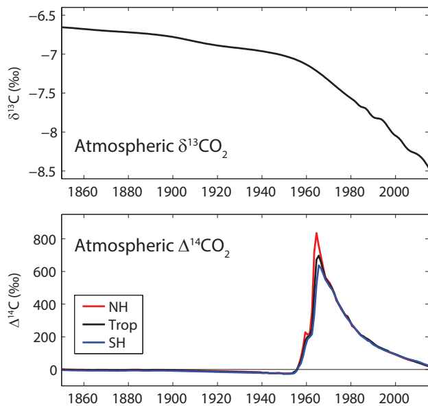
Figure 4. Carbon isotopes in atmospheric CO 2 for the historical period 1850–2014. Data for \delta^{13}\text{C} is from Law Dome, South Pole (Rubino et al., 2013), and Mauna Loa (Keeling et al., 2001) and includes smoothing of the observations. Data for \Delta^{14}\text{C} are compiled from Levin et al. (2010) and other sources (I. Levin, personal communication, 2016), following a similar data set used by Orr et al. (2000).
