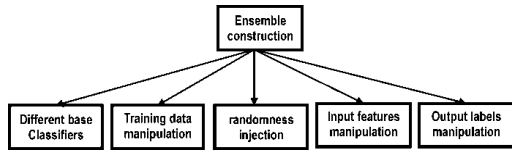
Fig. 2: Approaches for diverse classifier ensemble construction
