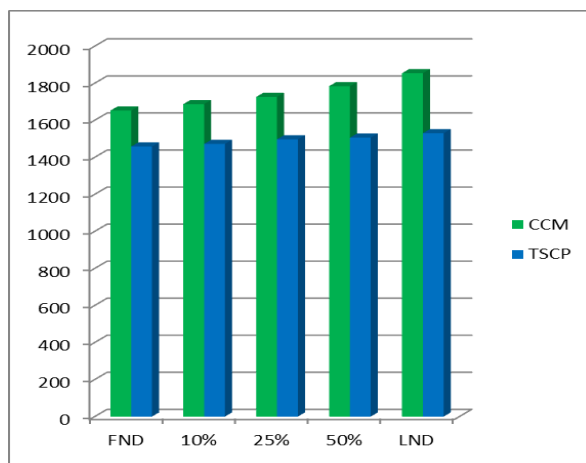
Figure 7: Network lifetime for CCM and TSCP with data fusing.
