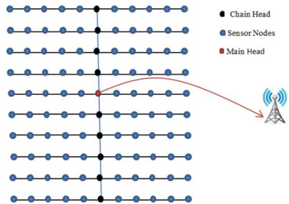
Figure 3: Chains constructed by TSCP protocol
