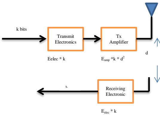
Figure 4: First Order Radio Model
