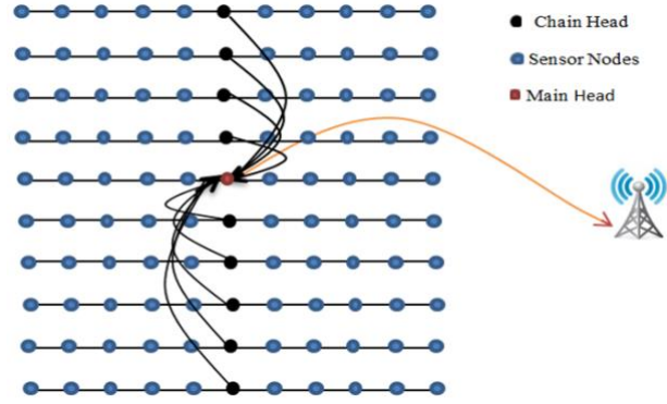
Figure 2: Chain and cluster formation in CCM
