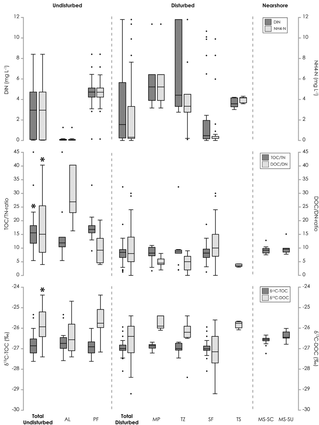
Fig. 5. Box-whisker plot displaying the DIN and NH 4 -N concentrations (upper box-whisker plots), TOC/TN- and DOC/DN-ratios (middle box-whisker plots), as well as δ 13 C-TOC and δ 13 C-DOC concentrations (lower box-whisker plots) in the undisturbed, disturbed and nearshore zone of the RTS; for visual reasons, the following outliers are not displayed: samples with DIN concentrations >12 \text{ mg L}^{-1} ( n = 2 in TZ, max: 77.3 \text{ mg L}^{-1} ; n = 5 in SF, max: 108.3 \text{ mg L}^{-1} ), TOC/TN-ratios >45 ( n = 1 in AL: 72; n = 1 in SF: 64), and DOC/DN-ratios >45 ( n = 3 in AL, max: 107; n = 2 in SF, max: 51).
