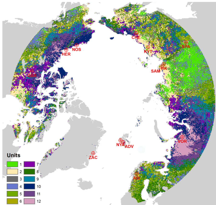
Figure 1: Circumpolar landscape units and location of PAGE21 sites
