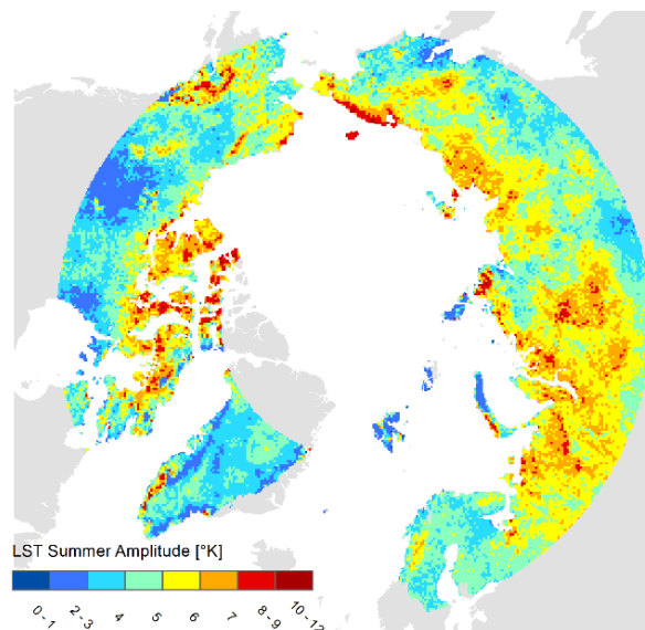
Figure 5: MODIS Landsurface temperature July/August Amplitude in Kelvin (derived from Duguay et al. 2014)
