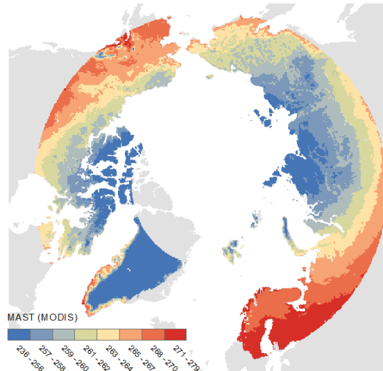
Figure 4: Mean annual surface temperature in Kelvin (derived from Duguay et al. 2014)
