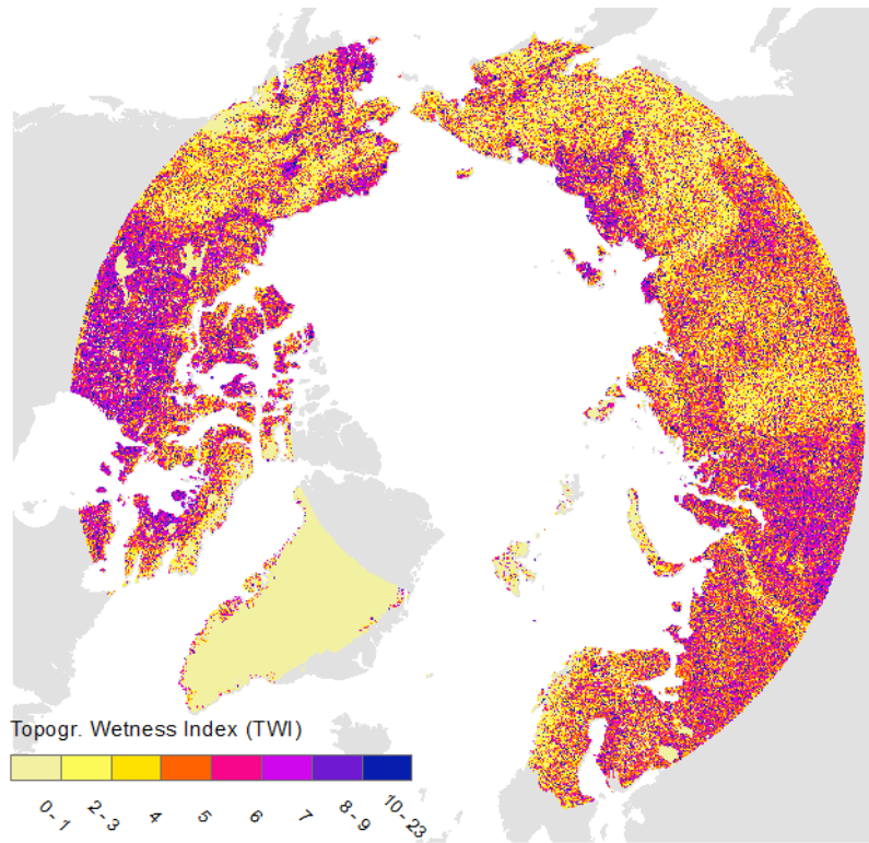
Figure 2: Circumpolar TWI (resampled to 25km 2 ; source Marthews et al. 2015)
