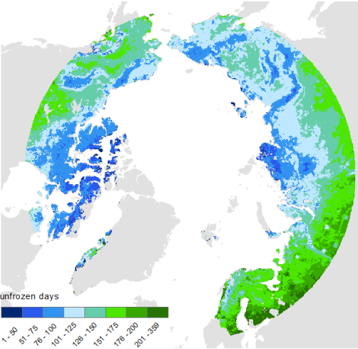
Figure 7: Length of unfrozen period in days (derived from Paulik et al. 2014)
