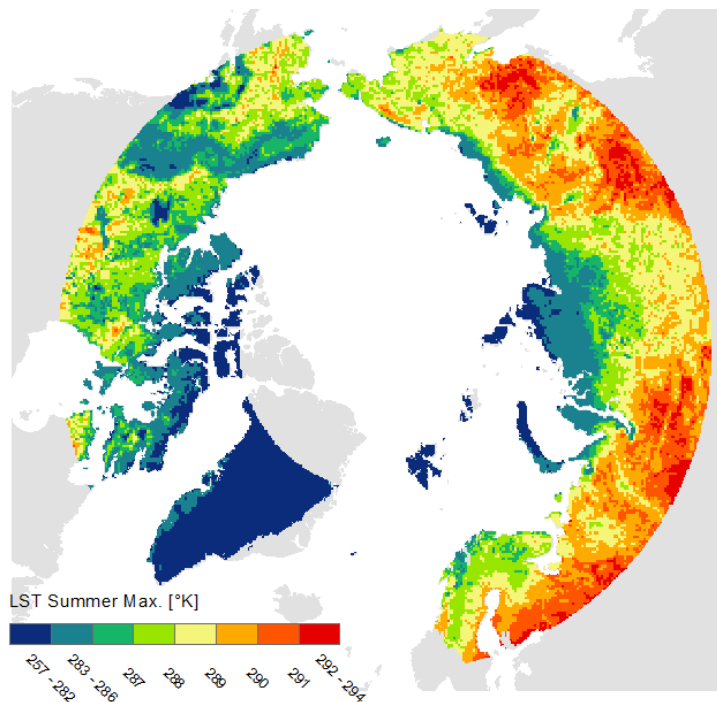
Figure 6: MODIS Landsurface temperature maximum in Kelvin (derived from Duguay et al. 2014)
