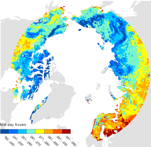
Figure 8: First day frozen (derived from Paulik et al. 2014)
