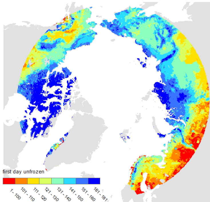
Figure 9: first day unfrozen (derived from Paulik et al. 2014)
