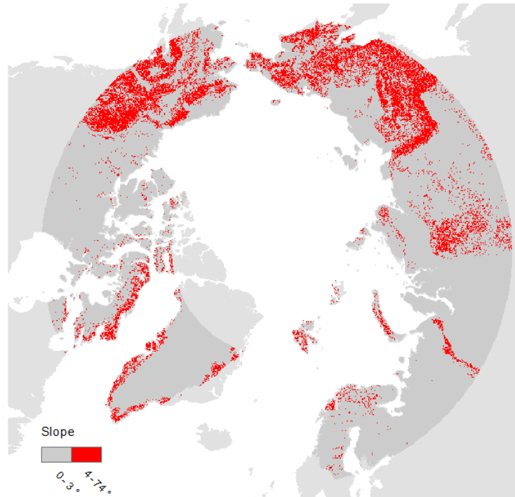
Figure 10: Slope units derived from Santoro et al. 2012
