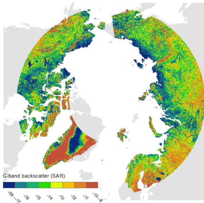
Figure 3: C-band winter backscatter from ENVISAT ASAR GM in dB (Widhalm et al. 2015)
