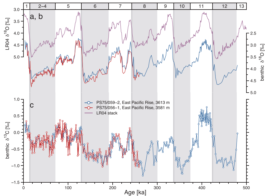
Figure 3. East Pacific Rise records from opposite ridge flanks. (a) LR04 benthic \delta^{18}\text{O} stack for stratigraphic reference. (b) Benthic \delta^{18}\text{O} records of cores PS75/059-2 and PS75/056-1. (c) Benthic \delta^{13}\text{C} records of cores PS75/059-2 and PS75/056-1; areas shaded in grey highlight glacial intervals.
