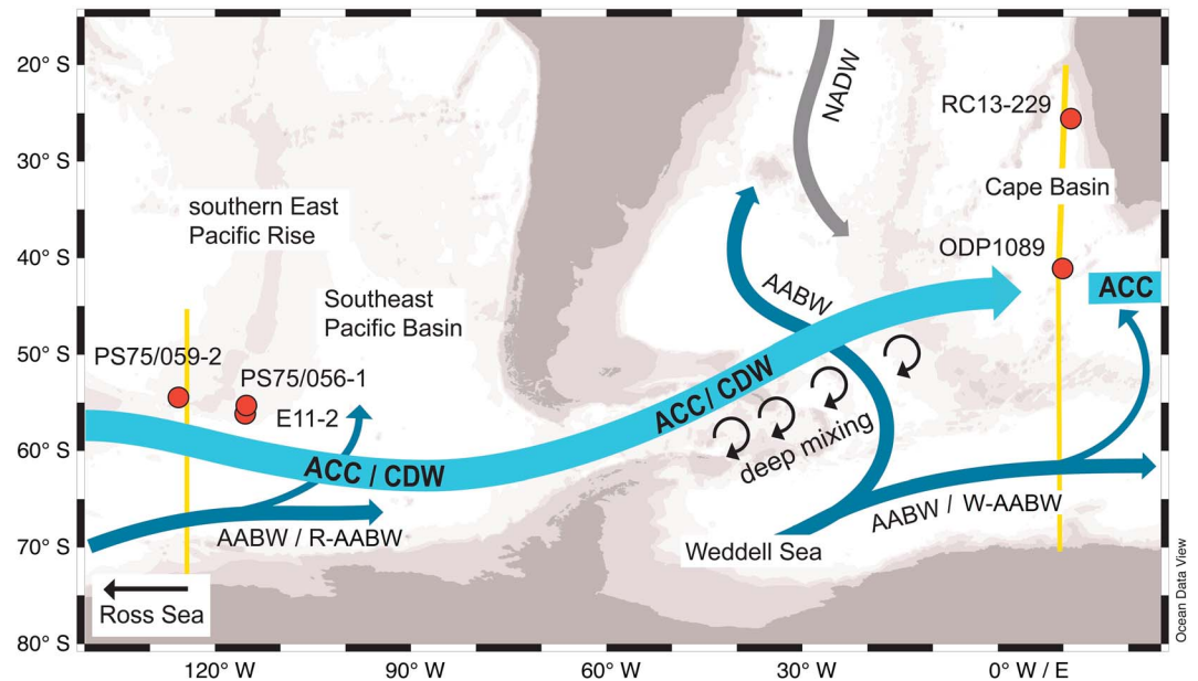
Figure 1. Map showing positions of discussed cores in the context of the modern deepwater hydrography; ocean and land topography is from Ocean Data View (ODV) [Schlitzer, 2012]; circles indicate position of cores discussed in this study; arrows show schematic flow path of major deepwater masses (CDW, Circumpolar Deep Water; AABW, Antarctic Bottom Water; NADW, North Atlantic Deep Water); two subtypes of AABW are indicated (R-AABW, Ross Sea derived AABW; W-AABW, Weddell Sea derived AABW); positions of the hydrographic sections displayed in Figure 2 are indicated as yellow lines.
