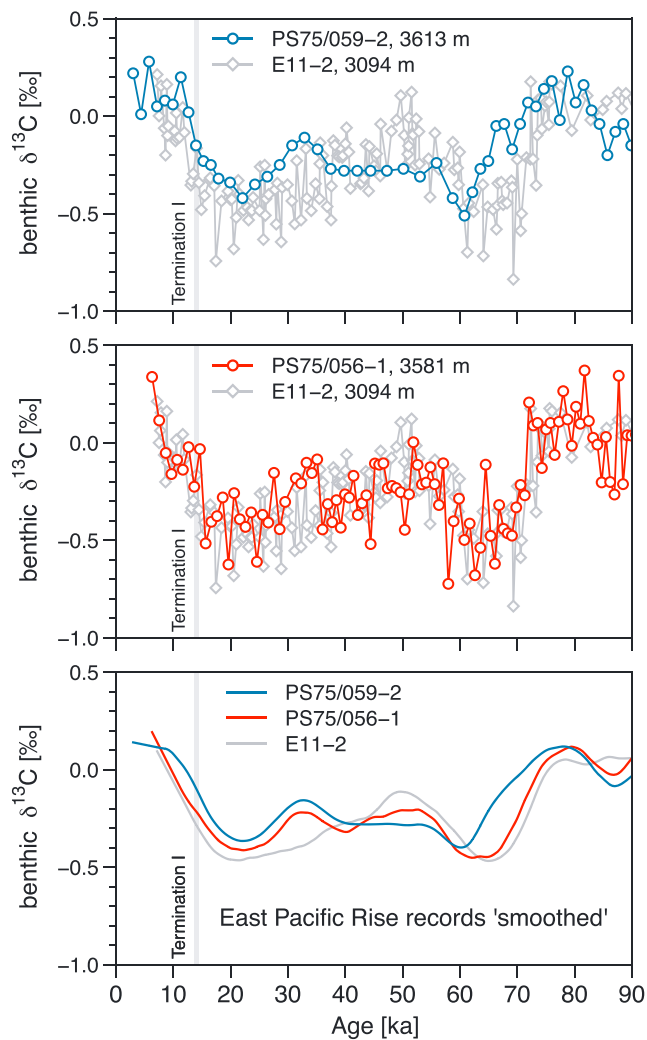
Figure 4. Comparison between benthic \delta^{13}\text{C} records from the East Pacific Rise. (a) Records PS75/059-2 and E11-2. (b) Records PS75/056-1 and E11-2. (c) Smoothed time series of records PS75/059-2, PS75/056-1, and E11-2, calculated by kernel method; gray vertical line marks the last glacial termination.
