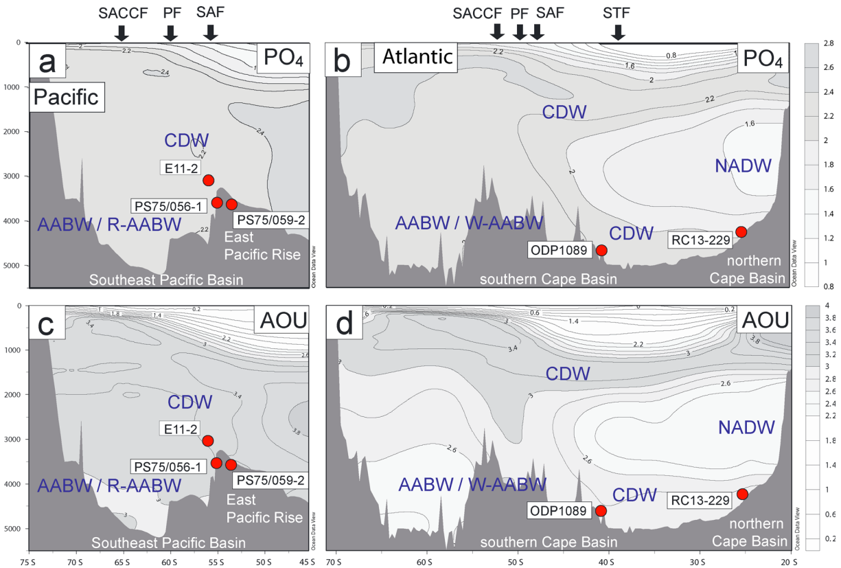
Figure 2. Modern \delta^{13}\text{C} ( \text{PO}_4^{3-} derived) and AOU distribution for (a and c) the Southeast Pacific and (b and d) the Southwest Atlantic; the position of sections are indicated in Figure 1 as yellow lines; the [\text{PO}_4^{2-}] and AOU are from the WOA09 (gridded) data compilation [Garcia et al., 2010a, 2010b]; for data visualization Ocean Data View (ODV) was used [Schlitzer, 2012]; circles indicate positions of cores discussed in this study; surface positions of Southern Ocean fronts are marked by arrows (STF, Subtropical Front; SAF, Subantarctic Front; PF, Polar Front; SACCF, Southern ACC Front), according Orsi et al. [1995]; Southern Ocean deepwater masses are indicated (CDW, Circumpolar Deep Water; AABW, Antarctic Bottom Water; NADW, North Atlantic Deep Water); two subtypes of AABW are indicated (R-AABW, Ross Sea derived AABW; W-AABW, Weddell Sea derived AABW).
