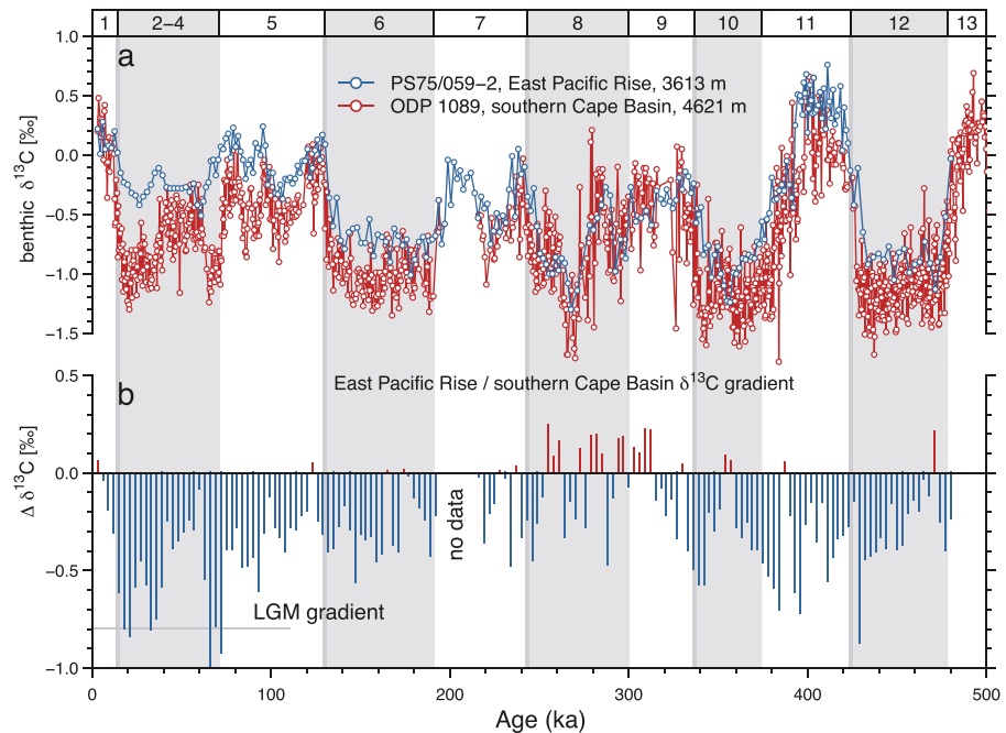
Figure 6. Comparison between East Pacific Rise and southern Cape Basin. (a) Benthic \delta^{13}\text{C} records PS75/059-2 and ODP Site 1089. (b) Difference between benthic \delta^{13}\text{C} records PS75/059-2 and ODP Site 1089 ( \Delta\delta^{13}\text{C} = \delta^{13}\text{C}_{\text{ODP Site 1089}} - \delta^{13}\text{C}_{\text{PS75/059-2}} ); the original time series ODP Site 1089 was smoothed using a 5-point moving average; before subtraction the smoothed time series ODP Site 1089 and the original time series PS75/059-2 were resampled in 3 ka spacing with linear interpolation between data points; the LGM gradient ( \sim -0.6\text{‰} ) is an average of the values between 18 ka and 24 ka; areas shaded in grey highlight glacial intervals; for resampling and smoothing the AnalySeries program was used [Paillard et al., 1996].
