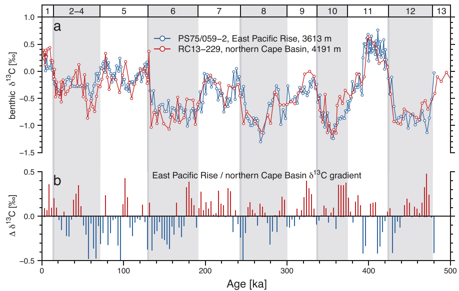
Figure 5. Comparison between East Pacific Rise and northern Cape Basin. (a) Benthic \delta^{13}\text{C} records PS75/059-2 and RC13-229. (b) Difference between benthic \delta^{13}\text{C} records PS75/059-2 and RC13-229 ( \Delta\delta^{13}\text{C} = \delta^{13}\text{C}_{\text{RC13-229}} - \delta^{13}\text{C}_{\text{PS75/059-2}} ); note that it shows any long-term trend; before subtraction the original time series were resampled in 3 ka spacing with linear interpolation between data points; areas shaded in grey highlight glacial intervals; for resampling the AnalySeries program was used [Paillard et al., 1996].
