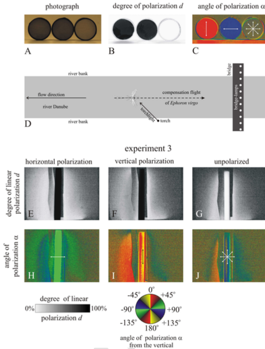
Fig. 2. Patterns of the degree of linear polarization d and the angle of polarization \alpha (clockwise from the vertical) of light sources used in field experiment 1 (A–C) and experiment 3 (E–J) measured with imaging polarimetry in the blue (450 nm) part of the spectrum. (A–C) Experiment 1: colour photograph (A), pattern of d (B) and \alpha (C) of the linearly polarizing and depolarizing filters. (D) Setup of experiment 1. (E–J) Experiment 3: patterns of d and \alpha of the light traps emitting horizontally polarized (E, H), vertically polarized (F, I) and unpolarized (G, J) light. The optical axis of the polarimeter was horizontal. Double-headed arrows show the local direction of polarization. (For interpretation of the references to colour in this figure legend, the reader is referred to the web version of this article.)
