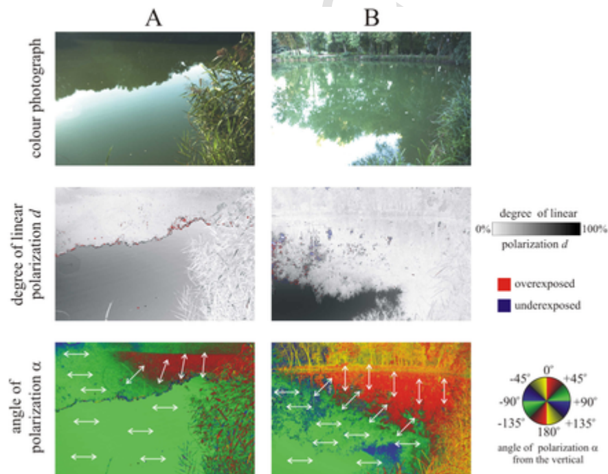
Fig. 6. Examples for two different edge regions of the same water body reflecting non-horizontally polarized light from the mirror image of riparian vegetation. (A) Reflection-polarization patterns of a water surface under a clear sky 1 h prior to sunset near the village Vác, Hungary measured with imaging polarimetry in the (450 nm) part of the spectrum. The polarimeter was pointed nearly towards the antisolar meridian, and its optical axis was tilted at -25^\circ from the horizontal. Double-headed arrows display the local direction of polarization of the water surface. (B) The polarimeter was pointed towards the antisolar meridian, and its optical axis was tilted at -37^\circ (Brewster angle) from the horizontal. Both polarimetric measurements were taken practically at the same time.
