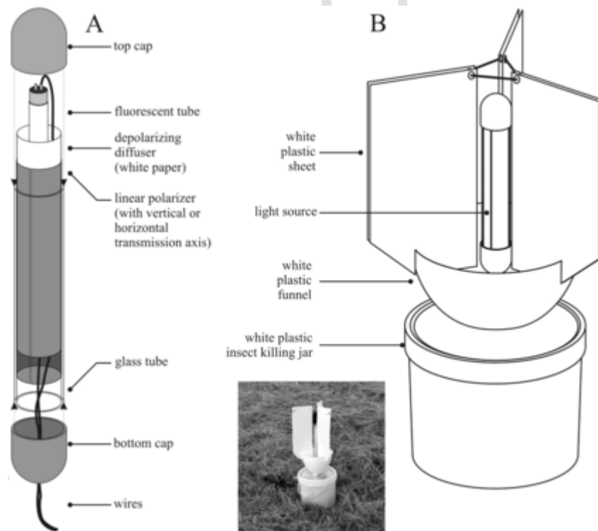
Fig. 3. (A) Structure of the light source of the traps used in experiment 3. In the case of the unpolarized light source the order of the polarizer and the depolarizing diffuser paper was reversed. (B) Structure of the light traps used in experiment 3. The inset is the photograph of a light trap.
