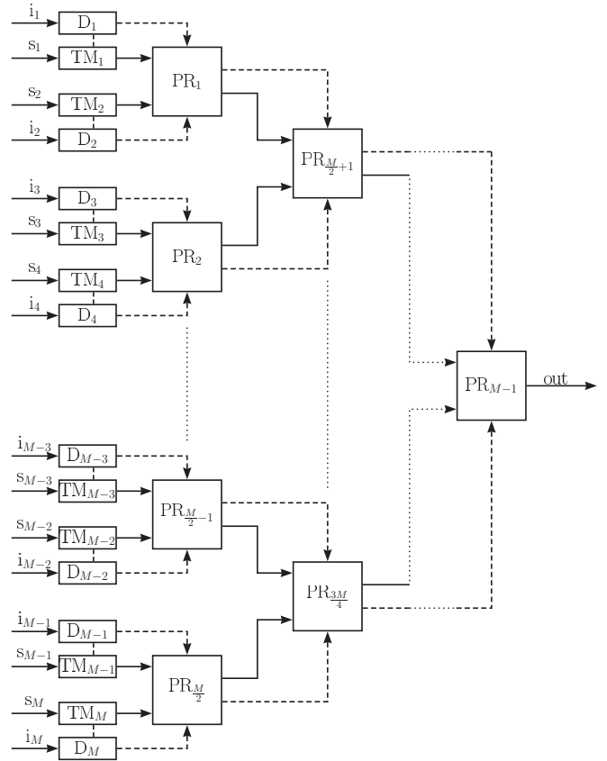
FIG. 1. Scheme of the combined multiplexer. TM_k is the k th time multiplexer, D_k 's are detectors, PR_k 's are photon routers. i_k and s_k denote the idler and signal arm of the k th nonlinear photon pair source. Dashed lines represent electronic control lines.
