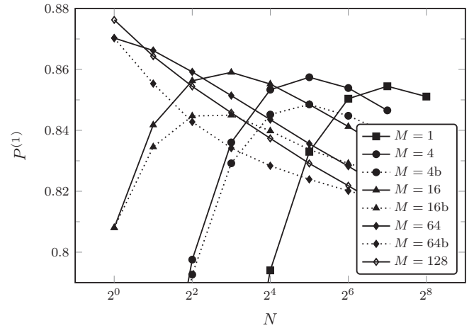
FIG. 3. The achievable maximal single-photon probability P^{(1)} at the optimal choice of the input mean photon number \lambda_{\text{opt}} as a function of the number of multiplexed time windows N on semilogarithmic scale for various numbers of spatially multiplexed time multiplexers M . Loss parameters are the following: V_r = 0.996 , V_t = 0.97 , V_p = 0.95 , V_{p0,S} = 0.996 , V_D = 0.9 , V_b = 1 . Points connected with continuous lines correspond to single-photon probabilities of combined multiplexers operating with the priority logic choosing the photon in the arm of the spatial multiplexer with the lowest loss and points with dotted lines to the one which simply routes the first arriving photon to the output.
