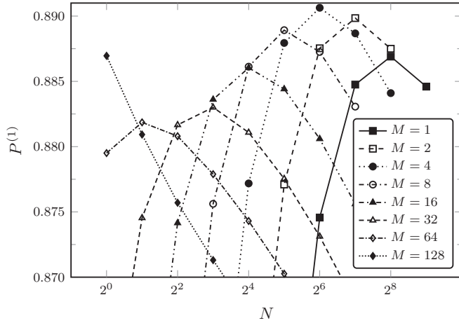
FIG. 6. The achievable maximal single-photon probability P^{(1)} at the optimal choice of the input mean photon number \lambda_{\text{opt}} as a function of the number of multiplexed time windows N on semilogarithmic scale for various numbers of spatially multiplexed time multiplexers M . Loss parameters are the following: V_r = 0.993 , V_{r,S} = 0.996 , V_t = 0.99 , V_{t,S} = 0.98 , V_p = 0.95 , V_{p0,S} = 0.995 , V_D = 0.9 , V_b = 1 .
