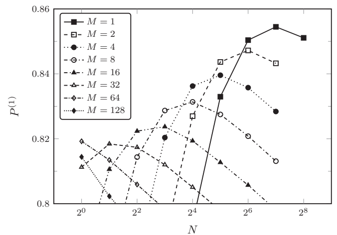
FIG. 4. The achievable maximal single-photon probability P^{(1)} at the optimal choice of the input mean photon number \lambda_{\text{opt}} as a function of the number of multiplexed time windows N on semilogarithmic scale for various numbers of spatially multiplexed time multiplexers M . Loss parameters are the following: V_r = 0.996 , V_t = 0.97 , V_p = 0.95 , V_{p0,S} = 0.985 , V_D = 0.9 , V_b = 1 .
