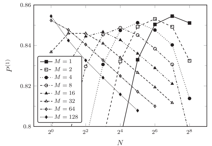
FIG. 5. The achievable maximal single-photon probability P^{(1)} at the optimal choice of the input mean photon number \lambda_{\text{opt}} as a function of the number of multiplexed time windows N on semilogarithmic scale for various numbers of spatially multiplexed time multiplexers M . Loss parameters are the following: V_r = V_{r,S} = 0.996 , V_t = V_{t,S} = 0.97 , V_p = 0.95 , V_{p0,S} = 0.9922 , V_D = 0.9 , V_b = 1 .
