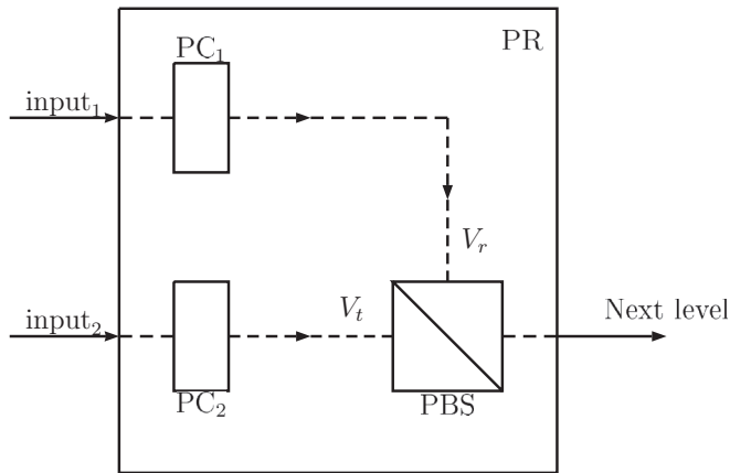
FIG. 2. Scheme of the bulk optical photon router. PCs denote Pockels cells and PBS is a polarizing beam splitter. V_r denotes the reflection efficiency and V_t the transmission efficiency of the PBS.
