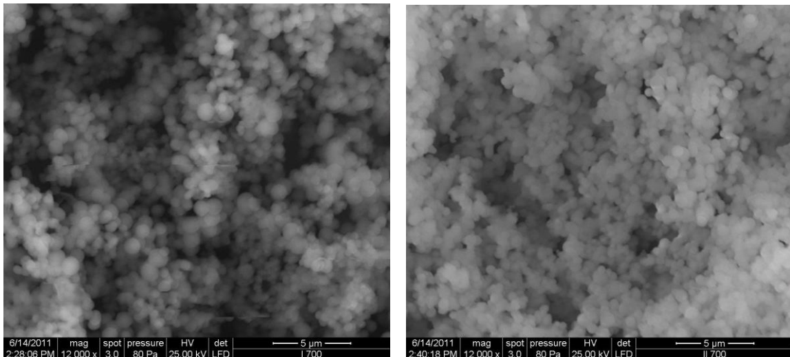
Figure 7. SEM micrographs of samples CTAB-NH3-700 (a) and CTAB-NaOH-700(b)
