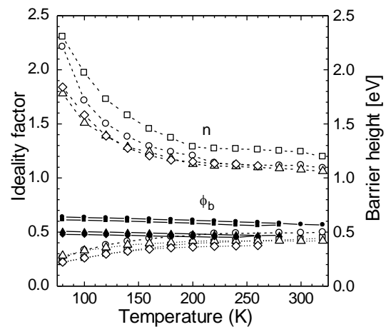
Fig. 2: The temperature dependence of ideality factor ( n ) and barrier height ( \phi_b ) evaluated from the capacitance-voltage (solid symbols) and current-voltage (open symbols) characteristics for four different InP Schottky junctions [21]
