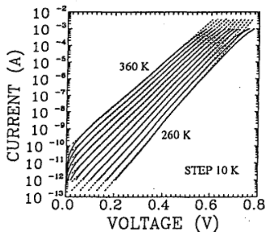
Fig. 1: Experimental current-voltage characteristics obtained in an Al/Al 0.75 Ga 0.25 As/Al 0.25 Ga 0.75 As Schottky junction as a function of temperature (solid lines) and fitted theoretical curves (dashed lines) [7,8]
