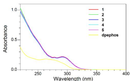
Fig. 2 Absorption spectra of complexes 1–5 and dpephos in methanol (10 \mu\text{M} ).
