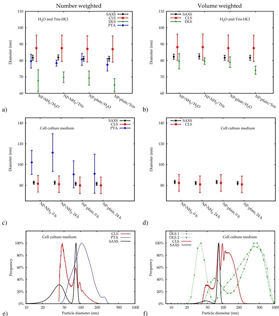
Fig. 10 Comparison of the results. The modal diameters determined for the dilution in water and Tris-HCl, directly after dispersion, are shown in (a) for number-weighted PSDs and in (b) for volume-weighted PSDs. The error bars denote expanded ( k = 2 ) uncertainties. The modal diameters measured in cell culture medium are displayed in (c) and (d), respectively. Here, the error bars for PTA and CLS do not include the additional unknown uncertainty contribution for measurements in complex media. Representative PSDs for the dispersion of NP-NH 2 in cell culture medium are shown in (e) and (f). The two results for DLS obtained from two consecutive runs of the same aliquot (dashed and dash-dotted green line) illustrate the repeatability issues of DLS in complex media.
