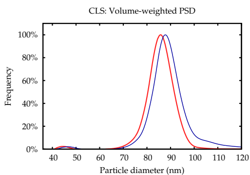
Fig. 1 TEM picture of the plain silica particles NP–plain (a). The scale bar represents a length of 500 nm. The PSD obtained from 250 particles in this image is shown in (b). Only particles with a diameter above 60 nm were counted. The volume-weighted size distribution obtained by CLS is shown in (c) for NP–plain (red line) and NP–NH 2 before ampouling (blue line)
