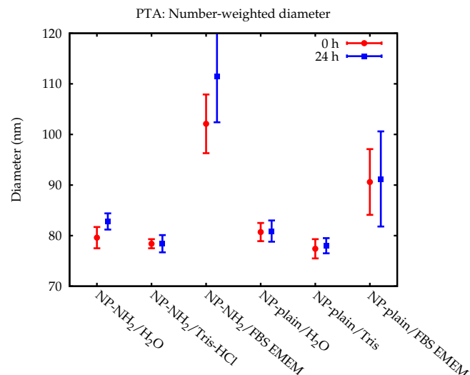
Fig. 9 Comparison of the number-weighted modal diameters obtained by PTA with standard uncertainties.
