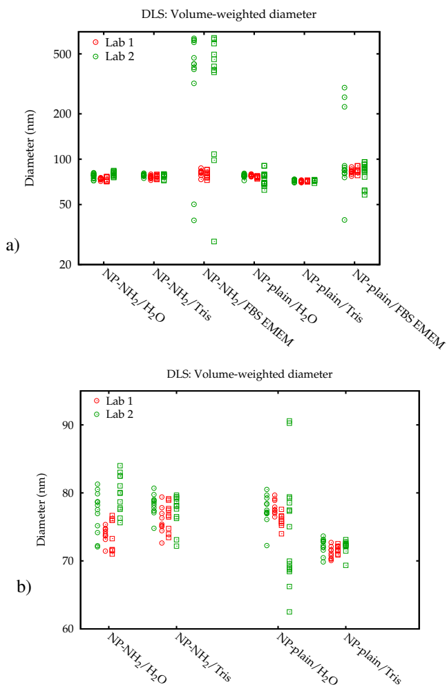
Fig. 3 Modal diameters obtained from volume-weighted PSD by DLS measurements in two laboratories. All individual values are plotted to illustrate the large range of the results from the same sample (a). Without the data in FBS EMEM, the DLS results are in the same scale for both media and laboratories (b). Round and square symbols display the values obtained immediately after dispersion, and after 24 h, respectively.
