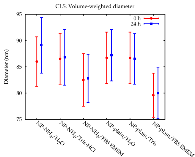
Fig. 5 Modal values for the primary peak of the volume-weighted PSDs obtained by CLS. The value was averaged over both laboratories. The error bars represent the combined standard uncertainty limited to the contributions relevant for comparing between CLS results.
