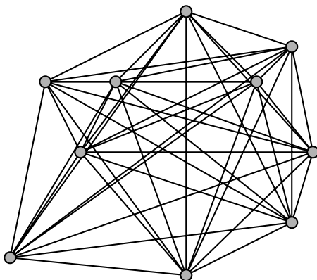
Figure 1. Can you group these ten points into four disjoint subsets such that the convex hulls of these subsets (which may amount to a point, an edge, or a triangle) have a point in common? A solution to this puzzle will be given below.
