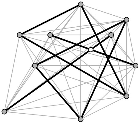
Figure 4. In this Tverberg partition for r = 4 , the marked intersection of two edges is contained inside the two bold triangles. This solves the puzzle at the beginning of the paper.
