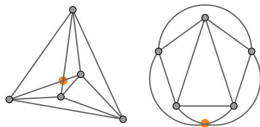
Figure 2. In every drawing of the complete graph K_5 , whether by straight lines or by curves, there are two non-adjacent edges that intersect.
