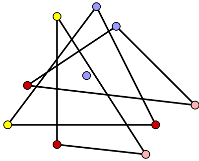
Figure 10. Does the Optimal Colored Tverberg Theorem fail for nonprime r , say for ten colored points in the plane, no four of the same color? The image is not a counterexample, because you can find that the point in the center is surrounded by three rainbow triangles.
