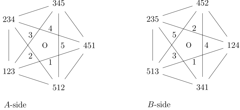
Figure 1: Any three of the 2-bodies, A_i \cup B_i , 0 \leq i \leq 5 , intersect, and they do not have a (1 - 1) -transversal
