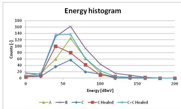
Fig 5 AE energy histograms of the tested samples
