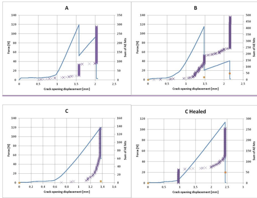
Fig 3 Recorded force and sum of AE hits curves of an unfilled (A), epoxy microcapsule filled (B), and a self-healing specimen before (C) and after healing (C Healed) as a function of crack opening displacement
