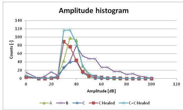
Fig 4 AE Amplitude histograms of the tested samples
