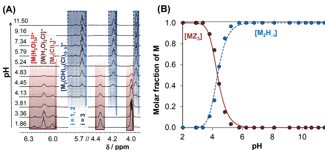
Fig. 6. pH-Dependent ^1\text{H} NMR spectra (A) and concentration distribution curves (B) of [\text{Ru}^{\text{II}}(\eta^6\text{-(2-phenoxyethanol)Z}_3)] ( \text{MZ}_3 where \text{Z} = \text{H}_2\text{O} or \text{Cl}^- ) in the presence of 0.1 M KCl. Notations for ^1\text{H} NMR spectra: non-hydrolyzed species: [\text{M}(\text{H}_2\text{O})_3]^{2+} , [\text{M}(\text{H}_2\text{O})_2\text{Cl}]^+ , [\text{M}_2(\text{Cl})_3]^+ formed by water/ \text{Cl}^- exchange (solid frame); hydrolyzed species: [\text{M}_2(\text{OH})(\text{Cl})_2]^+ , [\text{M}_2(\text{OH})_2\text{Cl}]^+ , [\text{M}_2(\text{OH})_3]^+ formed by \text{OH}^-/\text{Cl}^- exchange (dashed frame). Concentration distribution curves for [\text{MZ}_3] (solid line) and [\text{M}_2\text{H}_{-i}] hydroxido complexes (dashed line; i = 1, 2 or 3 ) calculated by the use of their overall stability constants, where \text{M} = \text{Ru}^{\text{II}}(\eta^6\text{-(2-phenoxyethanol)}) . Molar fractions based on the ^1\text{H} NMR peak integrals: [\text{MZ}_3] ( \bullet ) and summarized fractions for the hydroxido complexes ( \blacksquare ); \text{M} = \text{Ru}^{\text{II}}(\eta^6\text{-(2-phenoxyethanol)}) . \{c_{\text{M}} = 2 \text{ mM}; T = 25^\circ\text{C}; 10\% \text{ D}_2\text{O}\} .
