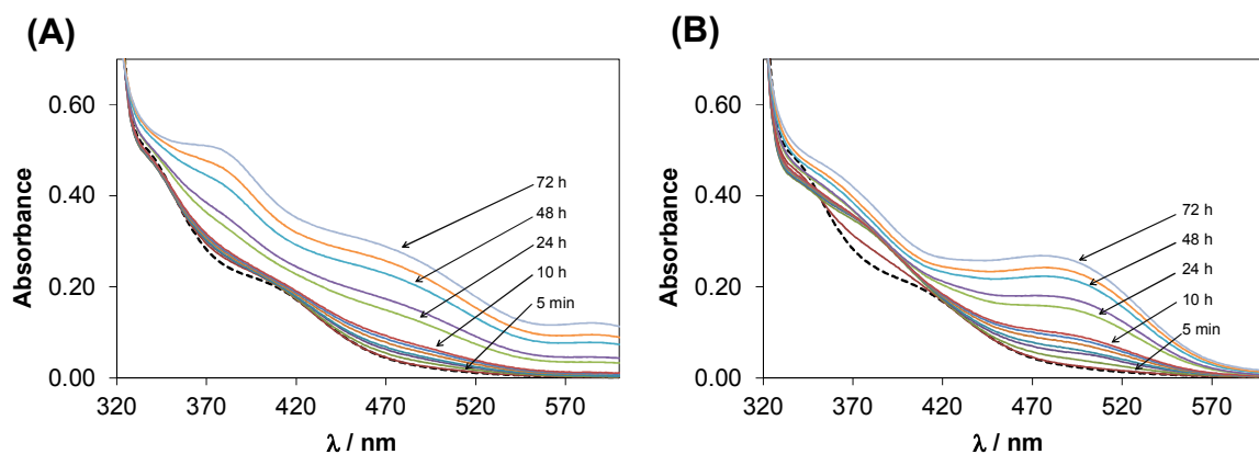
Fig. 8. Time dependent UV-Vis absorbance spectra of [\text{Ru}^{\text{II}}(\eta^6\text{-}(2\text{-phenoxyethanol}))(\text{bpy})\text{Z}] at pH 8.02→7.88 (A) and 9.58→9.05 (B) \{c_{\text{complex}} = 195 \mu\text{M}; I = 0.1\text{M} (\text{KCl}); T = 25 \text{ }^\circ\text{C}; Z = \text{H}_2\text{O}/\text{Cl}^-\} .
