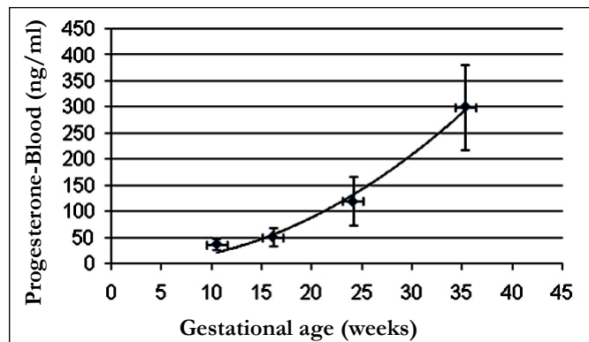
Figure 4. P4 in Blood of Pregnant Women.
