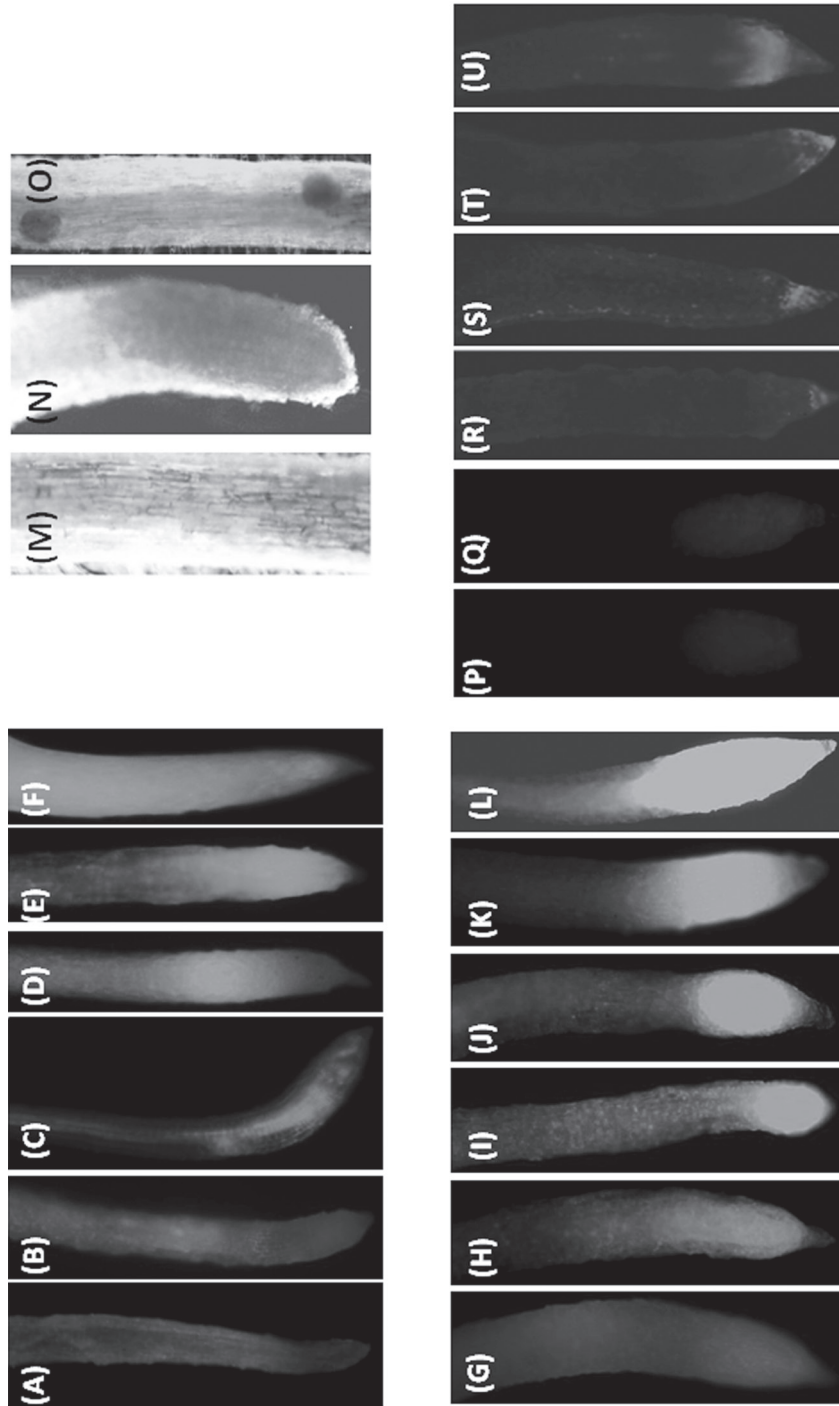
Fig. 2. (A–F) Superoxide detection using dihydroethidium in roots of wheat seedlings treated with 0, 50, 100, 200, 400 and 500 mg L -1 of ZnONPs respectively. (G–L) Detection of hydrogen peroxide accumulation using 3-(p-hydroxyphenyl) fluorescein treatment in roots of seedlings treated with 0, 50, 100, 200, 400 and 500 mg L -1 of ZnONPs respectively. (M, O) 500 mg L -1 of ZnONPs treated seedlings. Propidium iodide staining showing cell death in root tips of wheat seedlings (P) control, (Q–U) roots of seedlings grown in the presence of 50, 100, 200, 400 and 500 mg L -1 of ZnONPs respectively (4× magnification)
