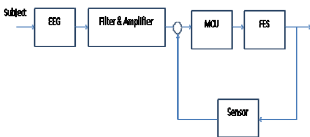
Figure 3: BCI-FES Control Scheme System
