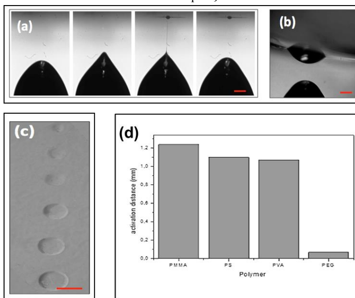
Figure 6.2. (a,b) Camera side view of the liquid dispensing onto a flat or a curved PE membrane, respectively; (c) microscope images of typical dispensed droplets; (d) distribution of the activation distance values for PE membranes made of different polymer solutions. Scale bars 200\mu\text{m} .
