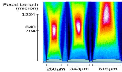
Figure 4.9: Focal lengths of PDMS microlenses with different diameters.
