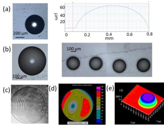
Figure 4.8: (a) Single PMMA microlens and corresponding profile, (b) PDMS microlens (left) and liner array of multiple lenses (right). Tilted interferometric fringe image (c), wavefront error (d) and 3-D image of the PMMA microlenses (e)
