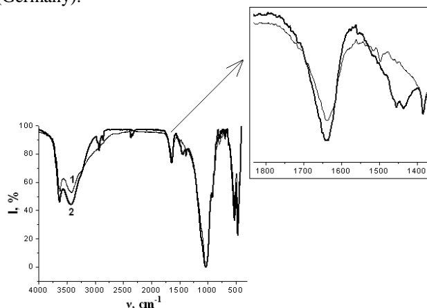
Fig. 2. IR spectra of the initial bentonite (curve 1) and the composite bentonite-PANI (curve 2)
