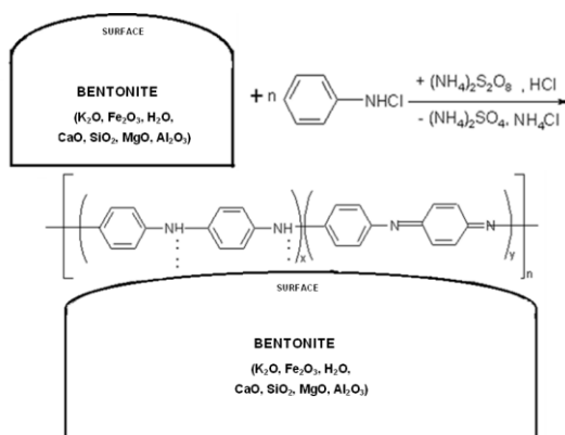
Fig. 1. Synthesis of composite bentonite-PANI
