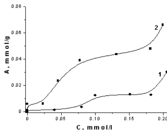
Fig. 11. Adsorption isotherms for Mo(VI) anions on bentonite (1) and bentonite immobilized by polyaniline (2) in distilled water
