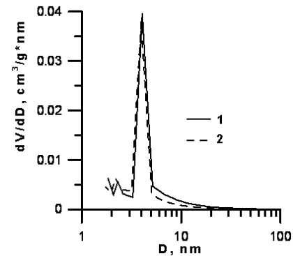
Fig. 5. Pore size distribution curves for the initial bentonite (curve 1) and the composite bentonite-PANI (curve 2)
