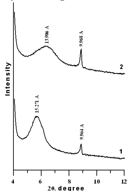
Fig. 6. XRD patterns of the initial bentonite (curve 1) and the composite bentonite-PANI (curve 2)
