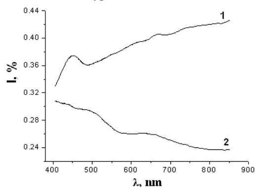
Fig. 3. DRES spectra of the initial bentonite (curve 1) and composite bentonite-PANI (curve 2)
