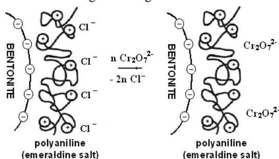
Fig. 8. Ion exchange mechanism of adsorption of ions
