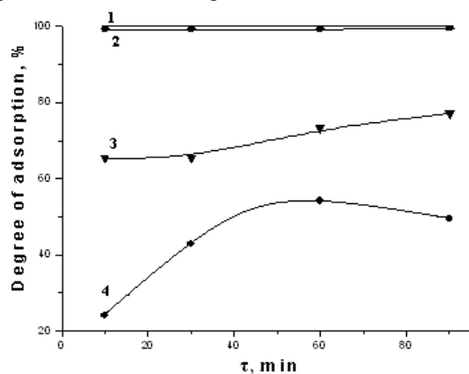
Fig. 9. Dependences of the degree of the adsorption of the anions of polyvalent metals upon the contact time on the composite bentonite immobilized by polyaniline: 1 – Cr(VI); 2 – W(VI); 3 – Mo(VI); 4 – V(V)
