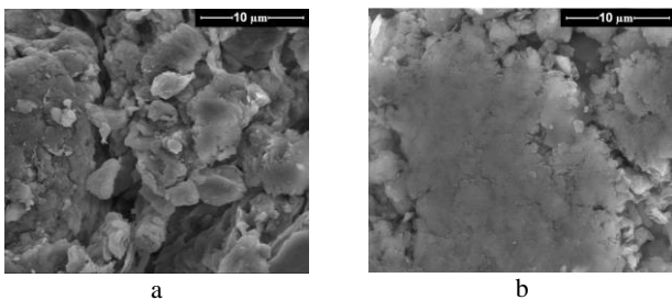
Fig. 7. Scanning electron spectroscopy (SEM) (magnification x5000) of a–the initial bentonite; b–the composite bentonite-PANI
