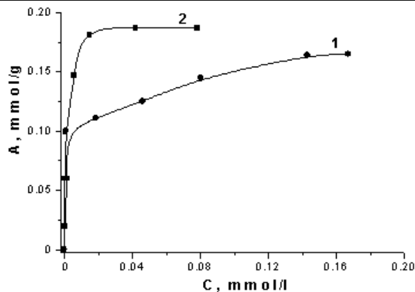
Fig. 10. Adsorption isotherms for Cr(VI) anions on bentonite (1) and bentonite immobilized by polyaniline (2) at pH = 1.7
