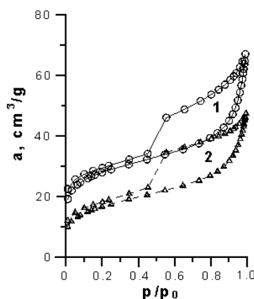
Fig. 4. Adsorption-desorption isotherms of nitrogen for the initial bentonite (curve 1) and the composite bentonite-PANI (curve 2)
