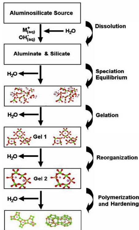
Figure 2.2: Conceptual model for geopolymerisation (Fernandez-Jimenez et al., 2006)
