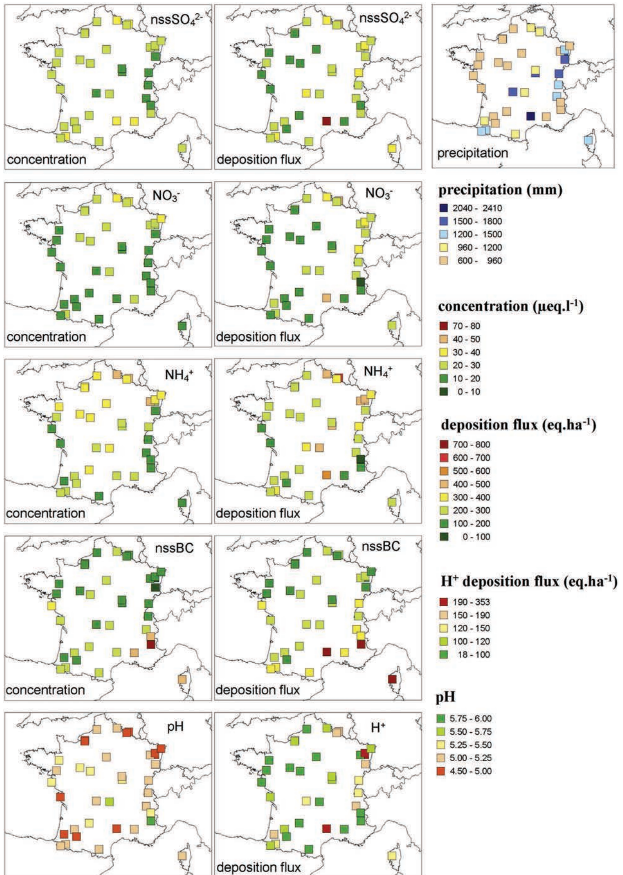
Fig. 2. Volume-weighted mean concentrations and deposition fluxes of non-sea-salt \text{SO}_4^{2-} , \text{NO}_3^- , \text{NH}_4^+ , non-sea-salt base cation, \text{H}^+ , mean pH (from volume-weighted mean \text{H}^+ concentrations) and annual precipitation in France for the period 1995–2007.
