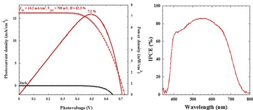
Figure 5. (J–V) curve under dark condition and under A.M. 1.5G illumination of flexible dye-sensitized solar cells composed of electrodeposited TiO 2 electrode of ca. 12 μm thick sensitized with C106 dye. The related IPCE action spectra is reported.
