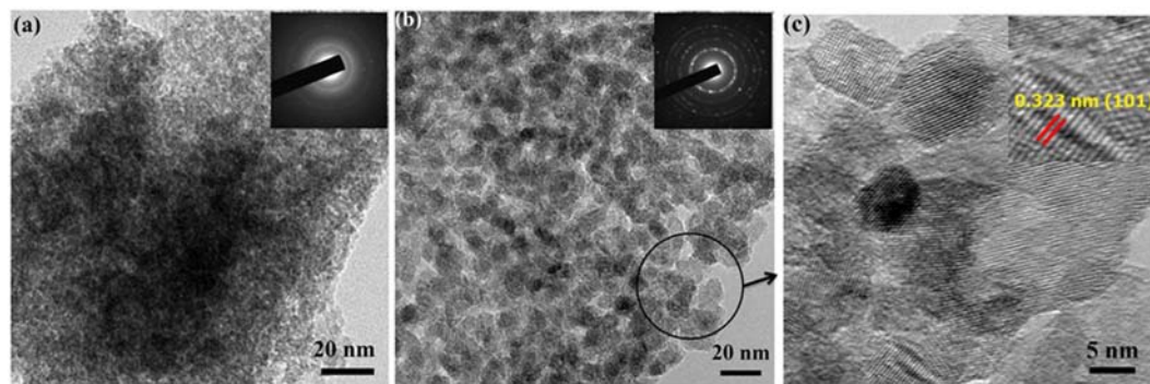
Figure 4. Comparison of TEM micrographs and SAED patterns for (a) as-prepared amorphous Ti(OH) 4 and (b) TiO 2 obtained after 15 days ageing in NH 4 F (aq) (c) HRTEM image of TiO 2 showing dominance of (101) diffraction planes.
