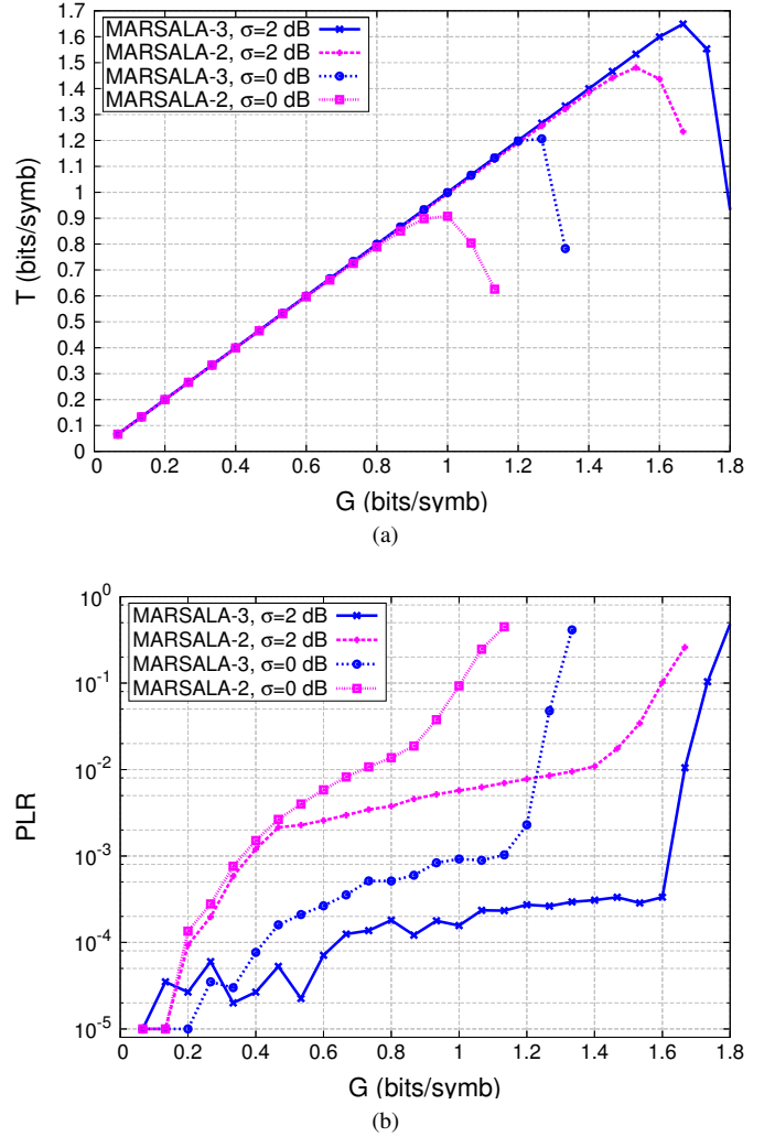
Fig. 4: Comparison between MARSALA-2 and MARSALA-3 with equi-powered packets and lognormally distributed packets power. QPSK modulation, DVB-RCS2 turbo code R = 1/3 , E_s/N_0 = 10 dB. (a) Throughput. (b) PLR.
