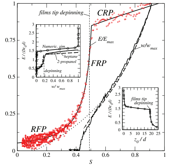
FIG. 3 (color online). Square tube drying kinetics with heptane [solid line from fits of z_0(t) , red circles from discrete derivatives, see text] and evolution of the corner film thickness w measured at a distance of one tube internal width d from tube entrance [solid line, the dotted line corresponds to the purely hydrostatic evolution, whereas the dashed line is deduced from a model of viscous flow in the film, see text, w_{\text{max}} = (\sqrt{2} - 1)(\frac{d}{3.77} - r_0) ]. The vertical dashed line marks the film tip depinning. The right-hand inset shows the drying kinetics as a function of z_0 computed numerically when the film thinning and depinning are due to gravity forces only. The left-hand inset shows the evolution of dimensionless evaporation flux as a function of w .
