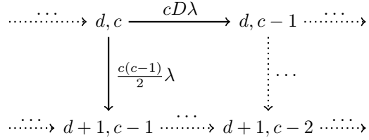
Figure 5: Chain transitions from a given state (d, c) . We observe that either we find one destination (d, c - 1) or we have a drop (d + 1, c - 1) . The rate at which we encounter a destination is increased by D when multiple destinations are available. The state (d + 1, c - 2) is included to show the progression of states.
