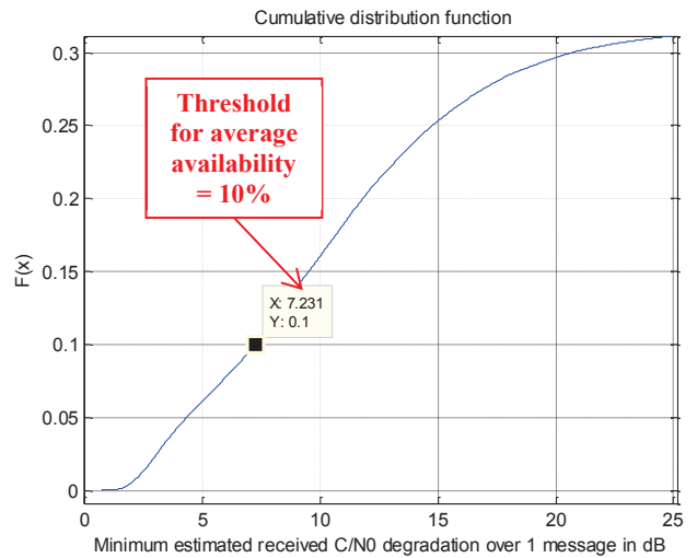
Figure 20: Cumulative distribution function of the degradation between the C_{pre-urban}/N_0 value and the minimum estimated received C/N_0 over 1 message, for C_{pre-urban}/N_0 = 25 dB-Hz and ideal phase estimation, with the DLR model
