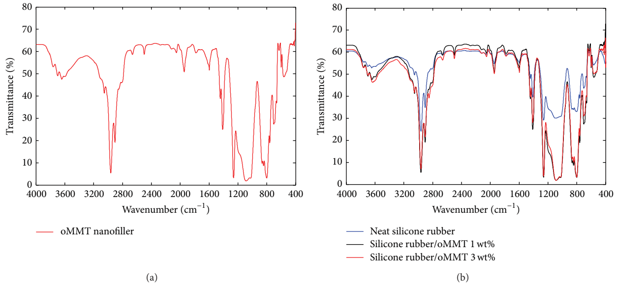
FIGURE 6: FTIR spectra. (a) oMMT nanofiller is denoted by the red line. (b) Neat silicone rubber is denoted by the blue line, silicone rubber-based nanocomposite (1 wt%) is denoted by the black line, and silicone rubber-based nanocomposite (3 wt%) is denoted by the red line.
