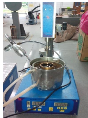
Figure 2 Penetration test
