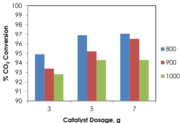
Figure 7 The trend plots of CO 2 conversion over Ru/Mn/Pr (5:30:65)/Al 2 O 3 catalyst calcined at various catalyst dosages
