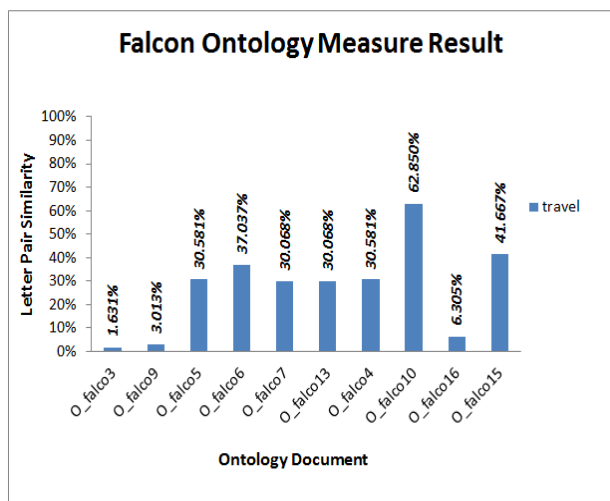
Figure 4 Graph of Falcons Ontology Measure Result
